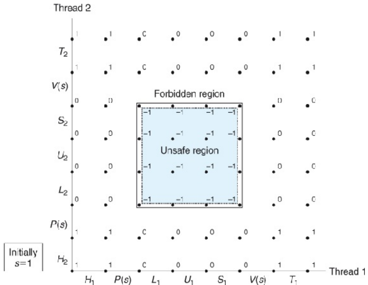
Figure 12.22 Using semaphores for mutual exclusion.
