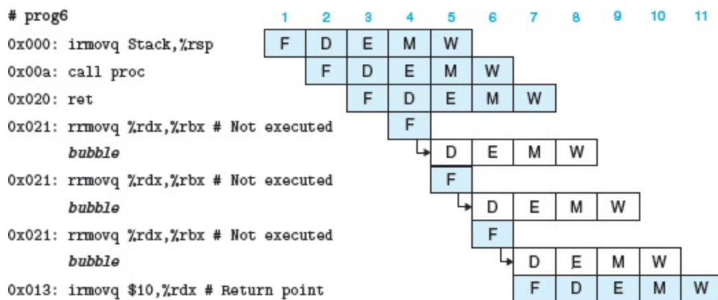
Figure 4.62 Detailed processing of the ret instruction.
