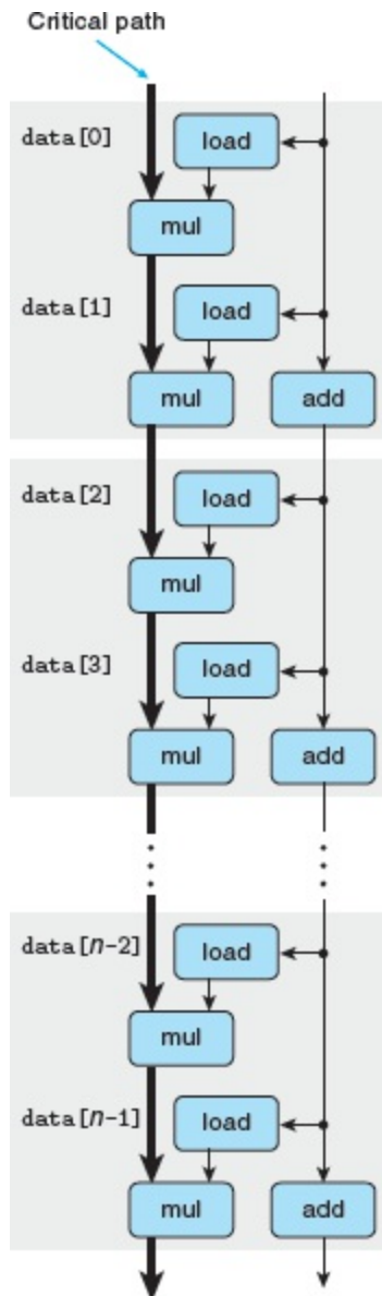
Figure 5.20 Data-flow representation of combine5 operating on a vector of length n .
