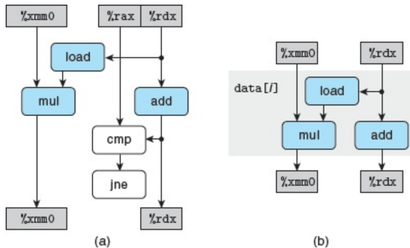
Figure 5.14 Abstracting combine4 operations as a data-flow graph.
