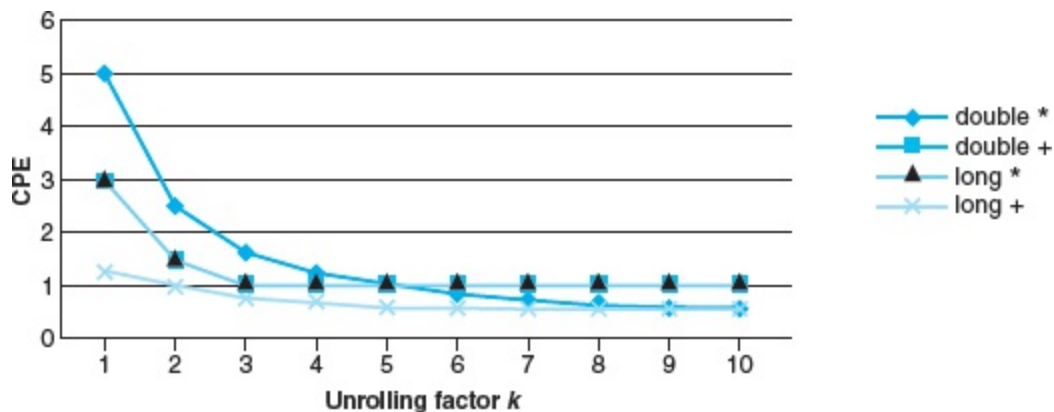
Figure 5.30 CPE performance for k \times 1a loop unrolling.
