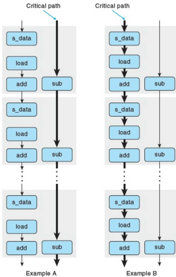
Figure 5.37 Data-flow representation of function write_read .
