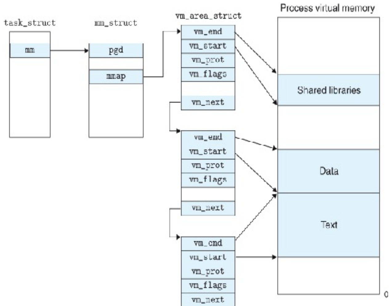
Figure 9.27 How Linux organizes virtual memory.
