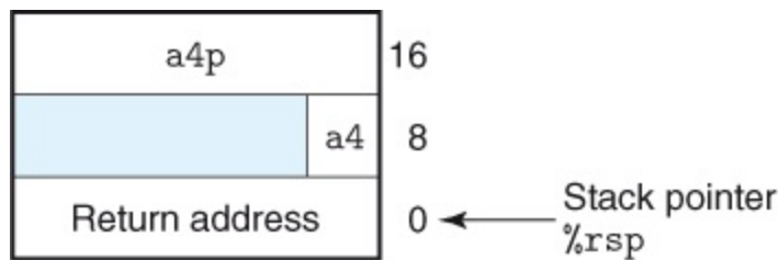
Figure 3.30 Stack frame structure for function proc .
