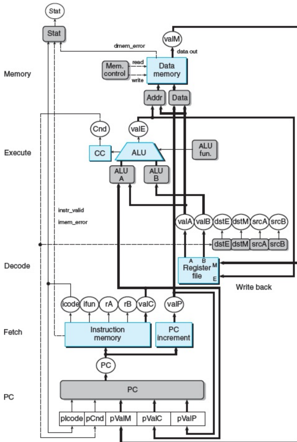
Figure 4.40 SEQ+ hardware structure.
