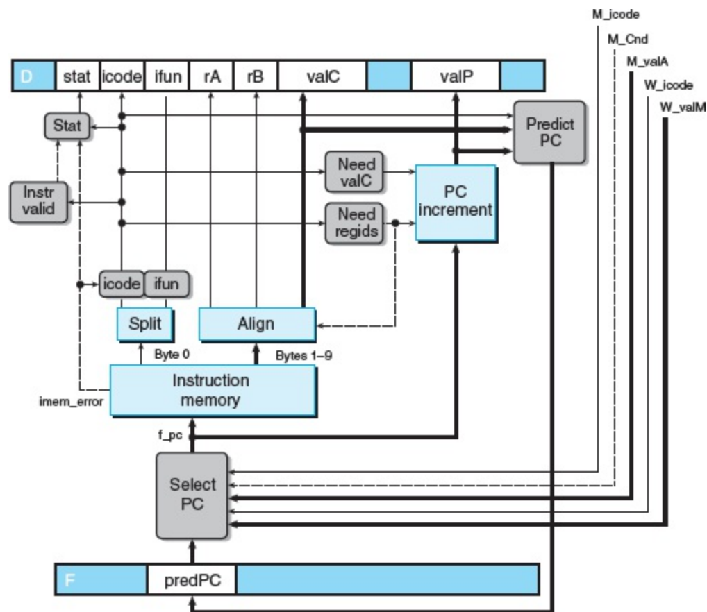
Figure 4.57 PIPE PC selection and fetch logic.
