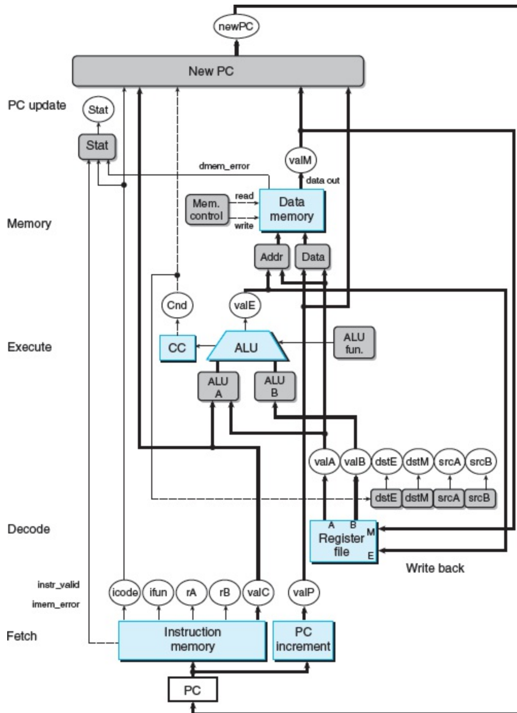
Figure 4.23 Hardware structure of SEQ, a sequential implementation.
