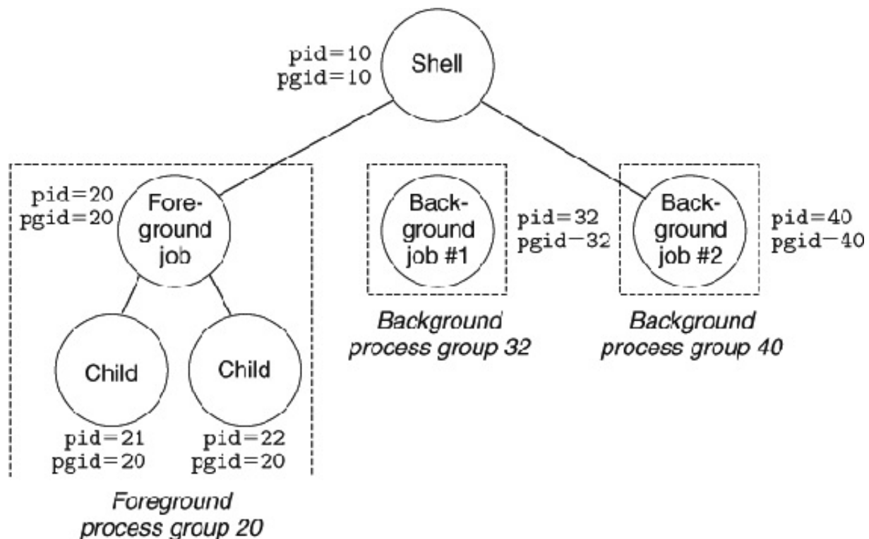
Figure 8.28 Foreground and background process groups.
