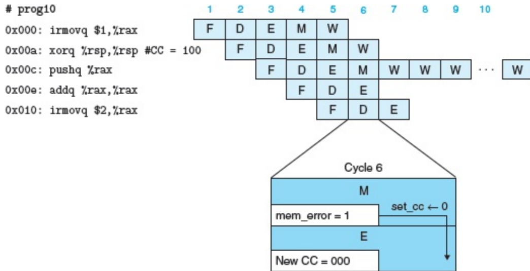
Figure 4.63 Processing invalid memory reference exception.
