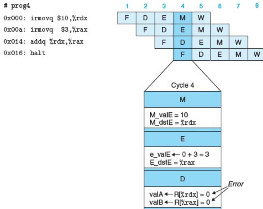
Figure 4.46 Pipelined execution of prog4 without special pipeline control.
