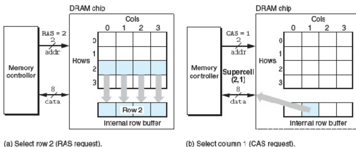
Figure 6.4 Reading the contents of a DRAM supercell.
