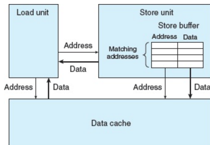
Figure 5.34 Detail of load and store units.
