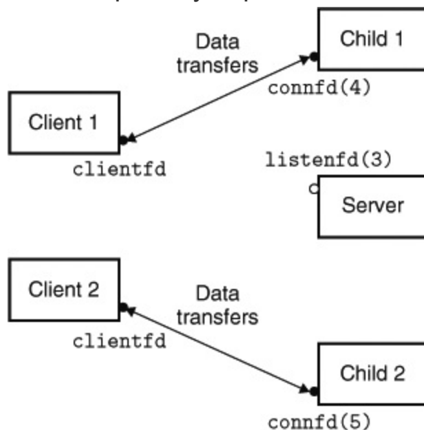
Figure 12.4 Step 4: Server forks another child to service the new client.
