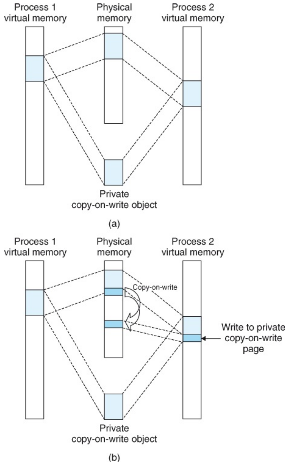
Figure 9.30 A private copy-on-write object.
