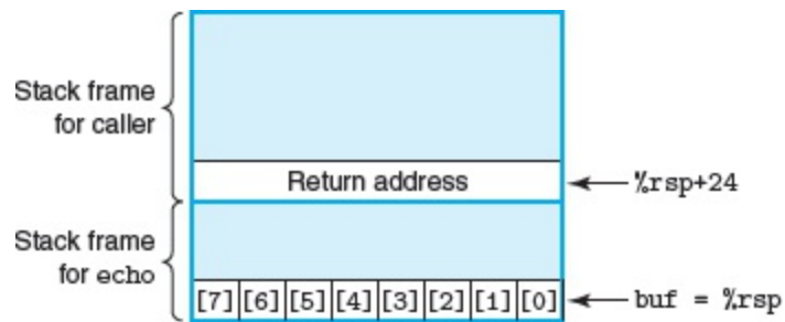
Figure 3.40 Stack organization for echo function.
