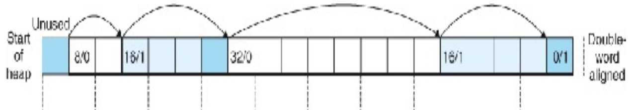
Figure 9.36 Organizing the heap with an implicit free list.
