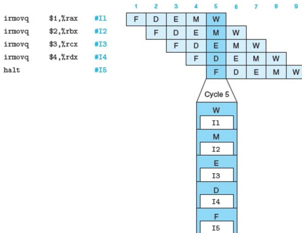
Figure 4.42 Example of instruction flow through pipeline.
