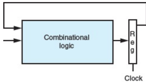
(a) Hardware: Unpipelined with feedback
