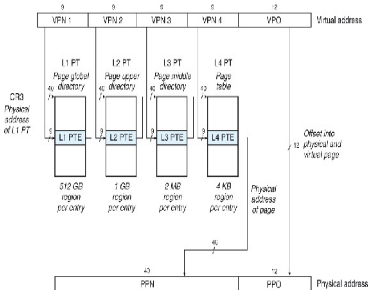
Figure 9.25 Core i7 page table translation.
