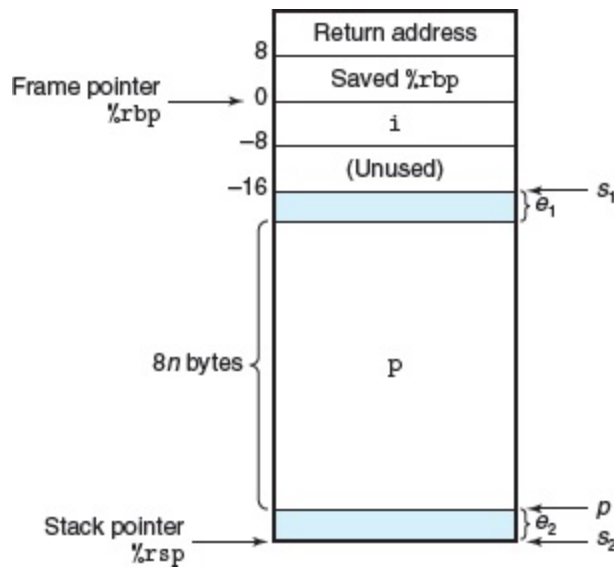
Figure 3.44 Stack frame structure for function vframe .
