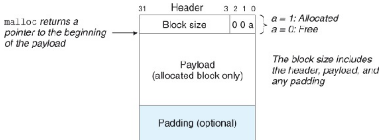
Figure 9.35 Format of a simple heap block.
