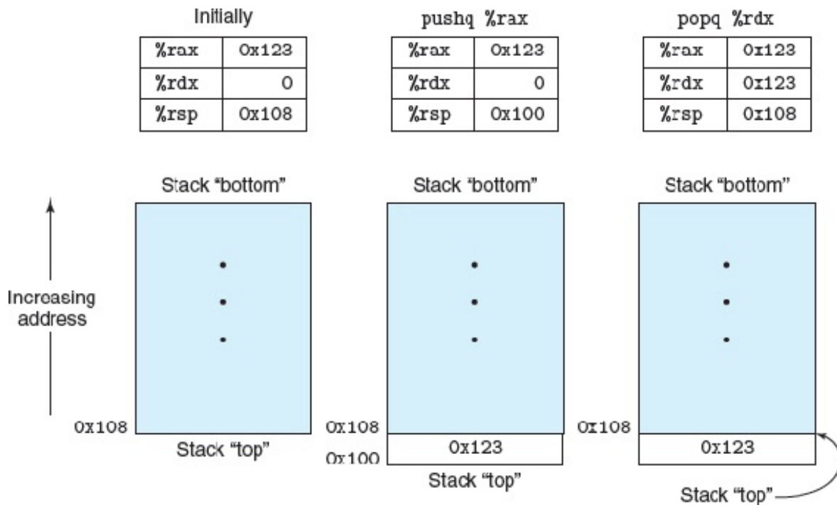
Figure 3.9 Illustration of stack operation.
