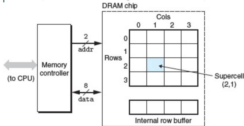
Figure 6.3 High-level view of a 128-bit 16 × 8 DRAM chip.
