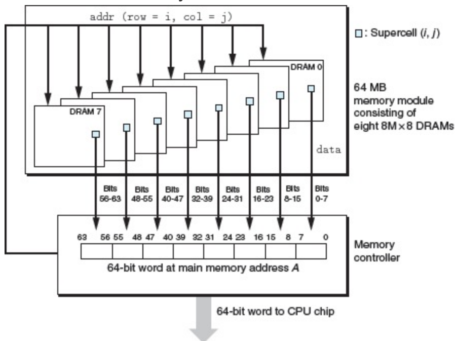
Figure 6.5 Reading the contents of a memory module.
