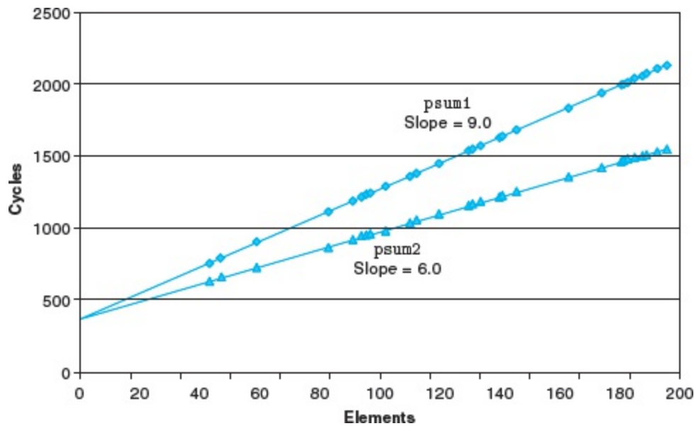
Figure 5.2 Performance of prefix-sum functions.
