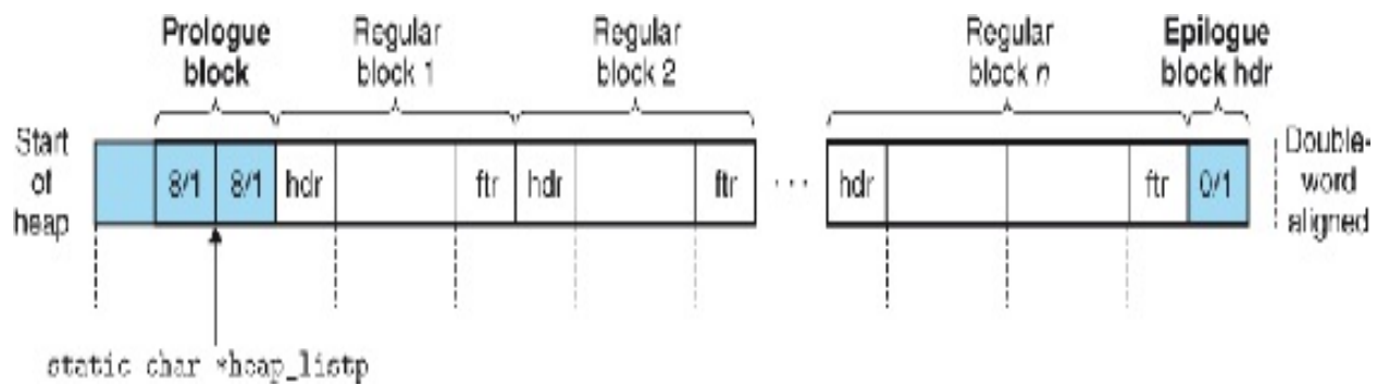
Figure 9.42 Invariant form of the implicit free list.
