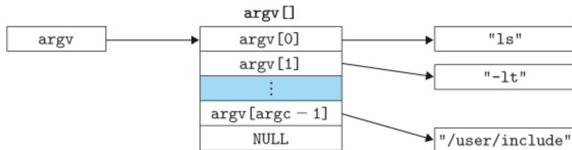
Figure 8.20 Organization of an argument list.
