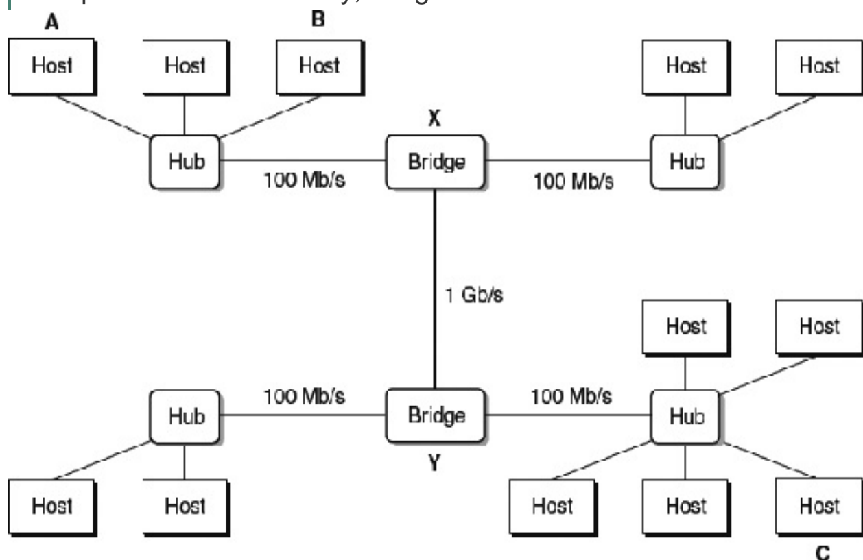
Figure 11.4 Bridged Ethernet segments.
