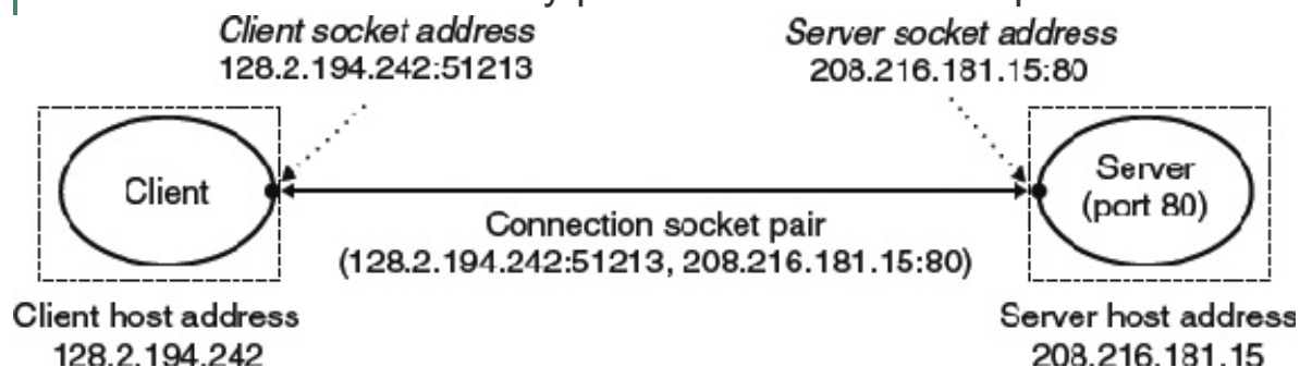
Figure 11.11 Anatomy of an Internet connection.
