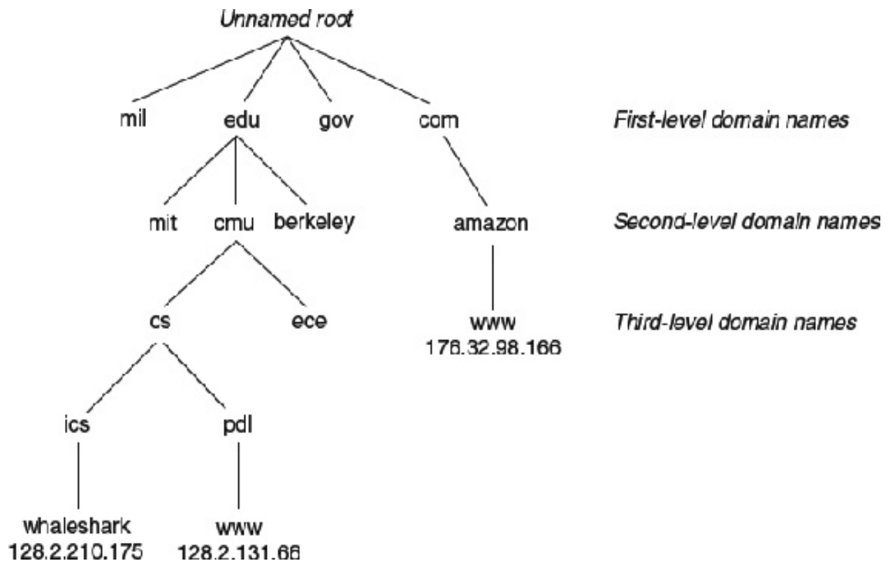
Figure 11.10 Subset of the Internet domain name hierarchy.
