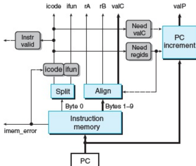
Figure 4.27 SEQ fetch stage.
