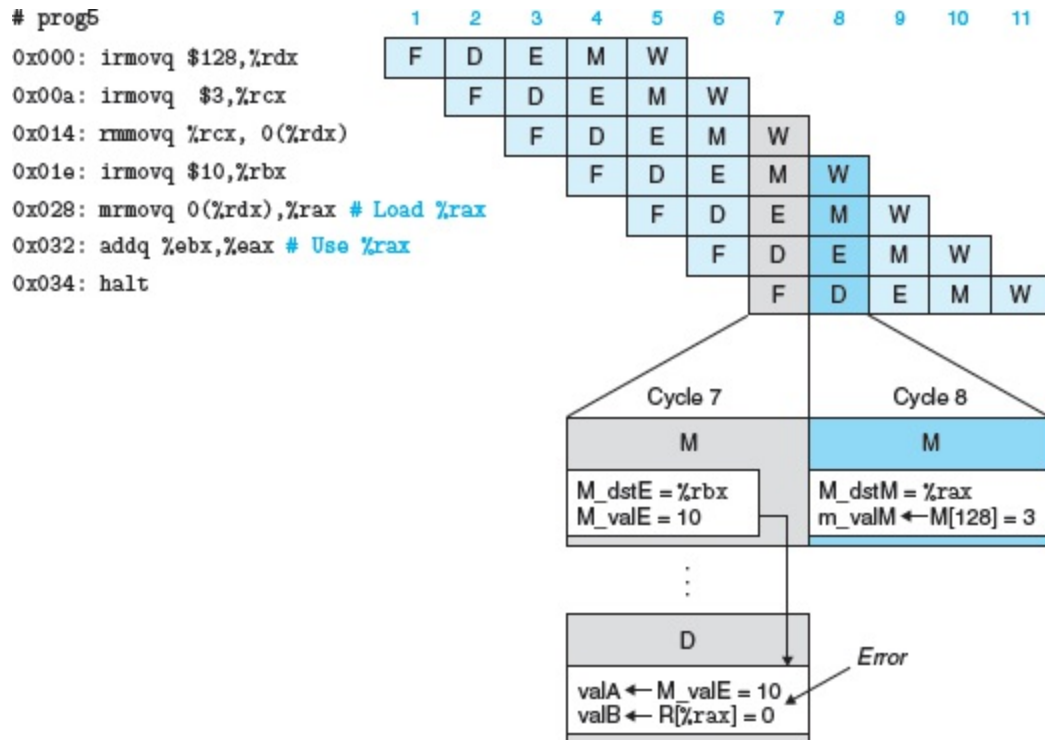
Figure 4.53 Example of load/use data hazard.
