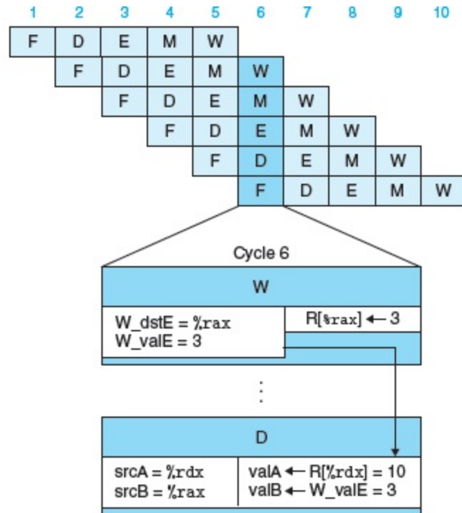
Figure 4.49 Pipelined execution of prog2 using forwarding.
