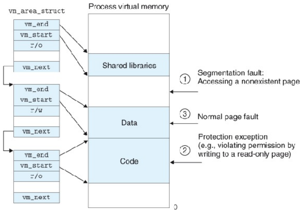
Figure 9.28 Linux page fault handling.
