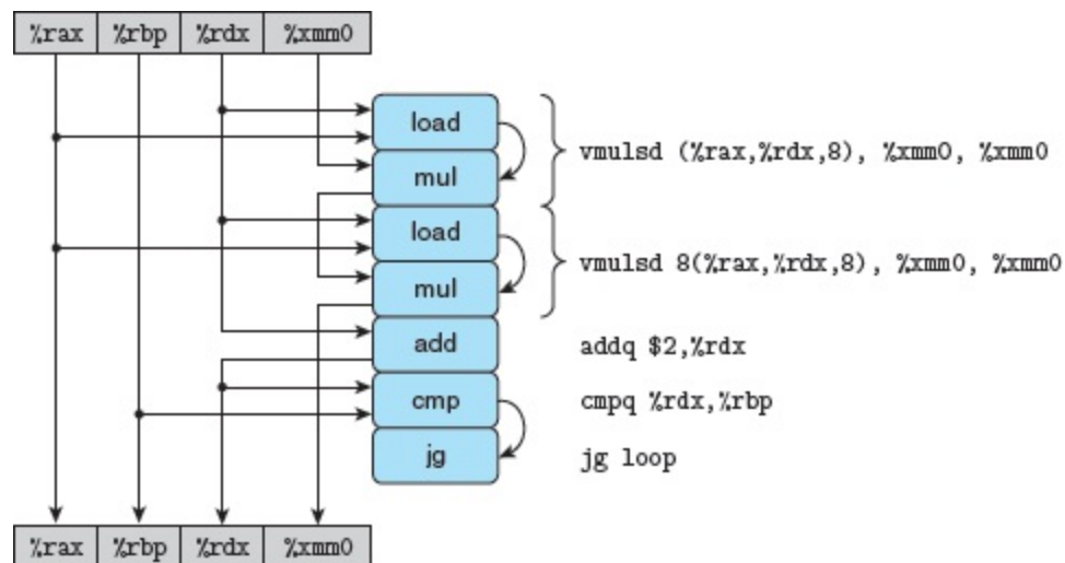
Figure 5.18 Graphical representation of inner-loop code for combine5 .
