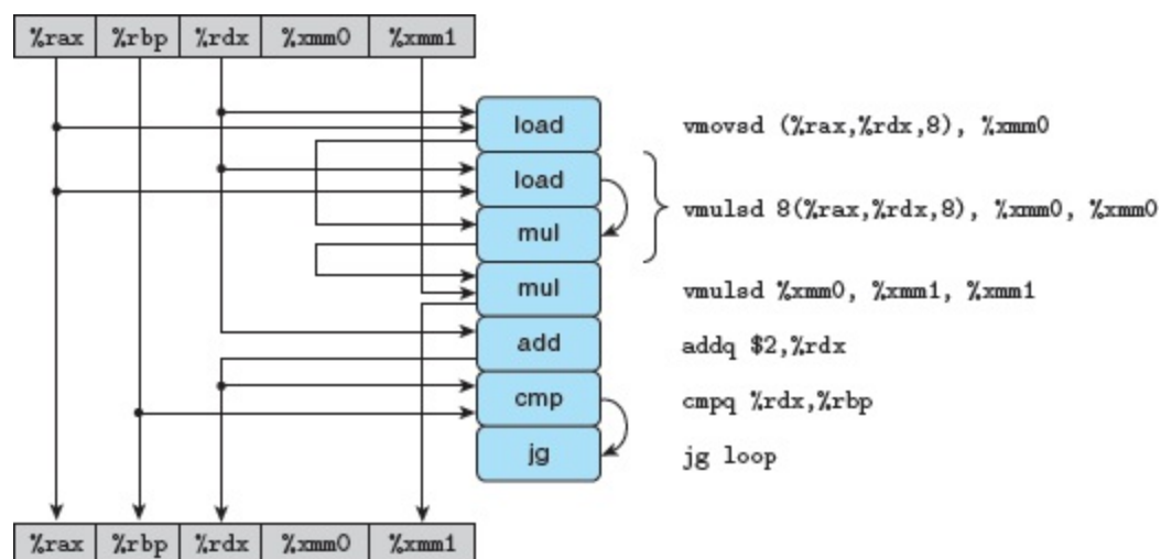
Figure 5.27 Graphical representation of inner-loop code for combine7 .
