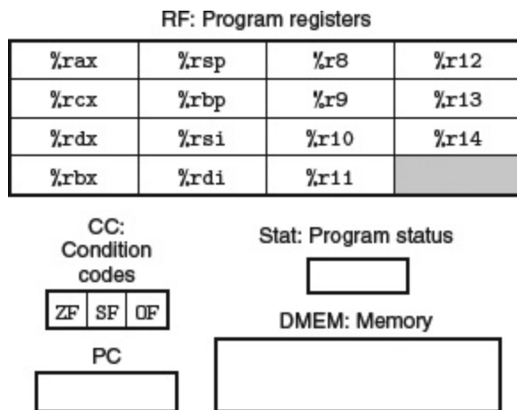
Figure 4.1 Y86-64 programmer-visible state.
