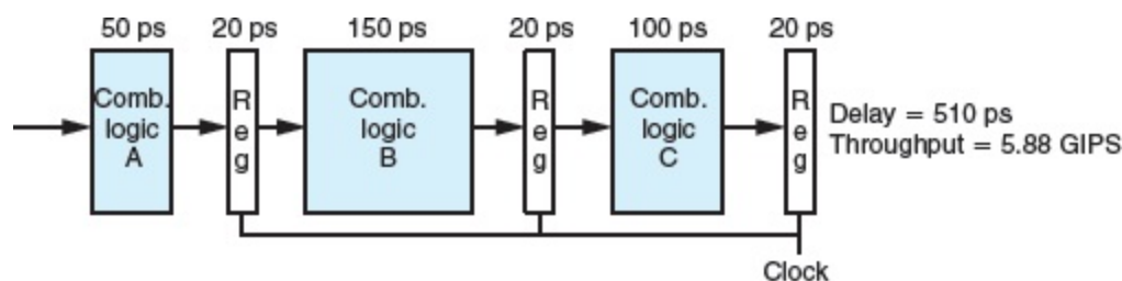
(a) Hardware: Three-stage pipeline, nonuniform stage delays
