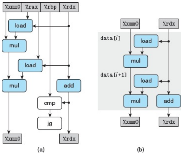
Figure 5.19 Abstracting combine5 operations as a data-flow graph.
