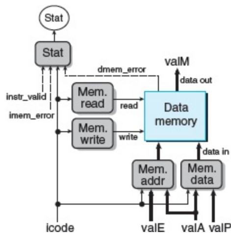
Figure 4.30 SEQ memory stage.
