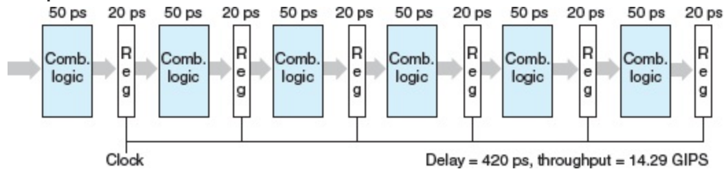
Figure 4.37 Limitations of pipelining due to overhead.
