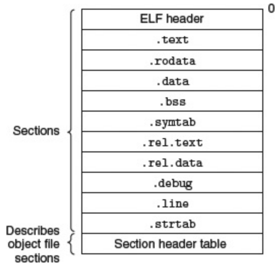
Figure 7.3 Typical ELF relocatable object file.
