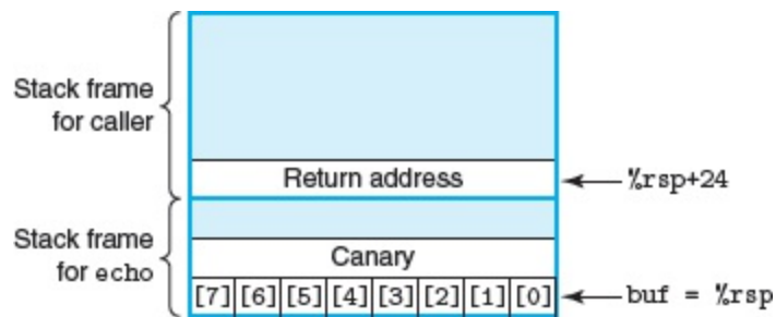
Figure 3.42 Stack organization for echo function with stack protector enabled.
