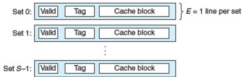
Figure 6.27 Direct-mapped cache ( E = 1 ).
