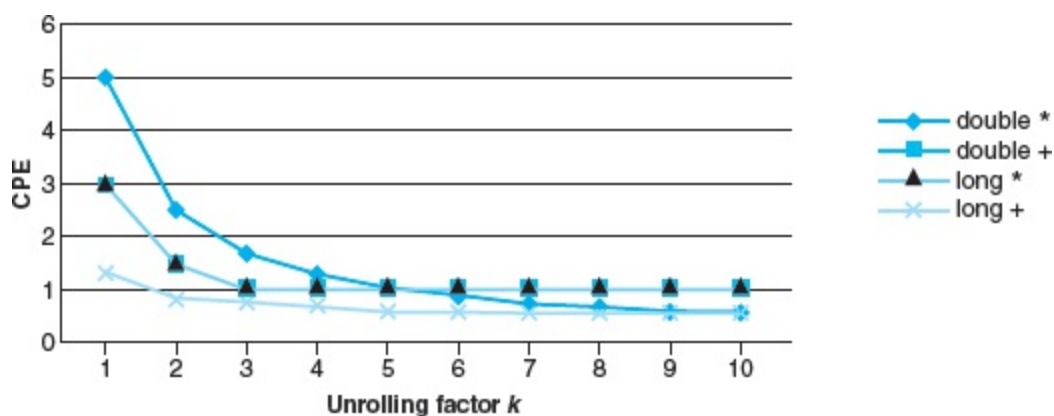
Figure 5.25 CPE performance of k \times k loop unrolling.
