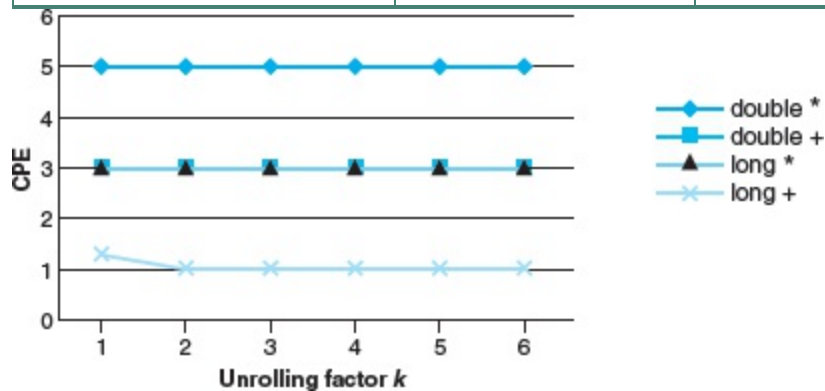
Figure 5.17 CPE performance for different degrees of k \times 1 loop unrolling.
