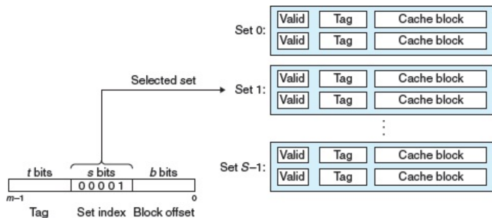
Figure 6.33 Set selection in a set associative cache.
