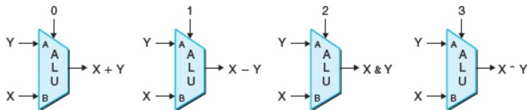
Figure 4.15 Arithmetic/logic unit (ALU).
