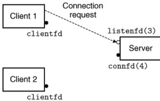
Figure 12.1 Step 1: Server accepts connection request from client.
