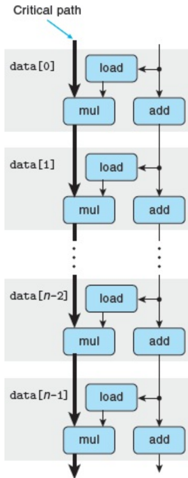
Figure 5.15 Data-flow representation of computation by n iterations of the inner loop of combine4 .
