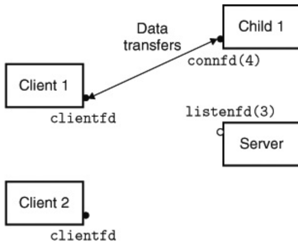
Figure 12.2 Step 2: Server forks a child process to service the client.
