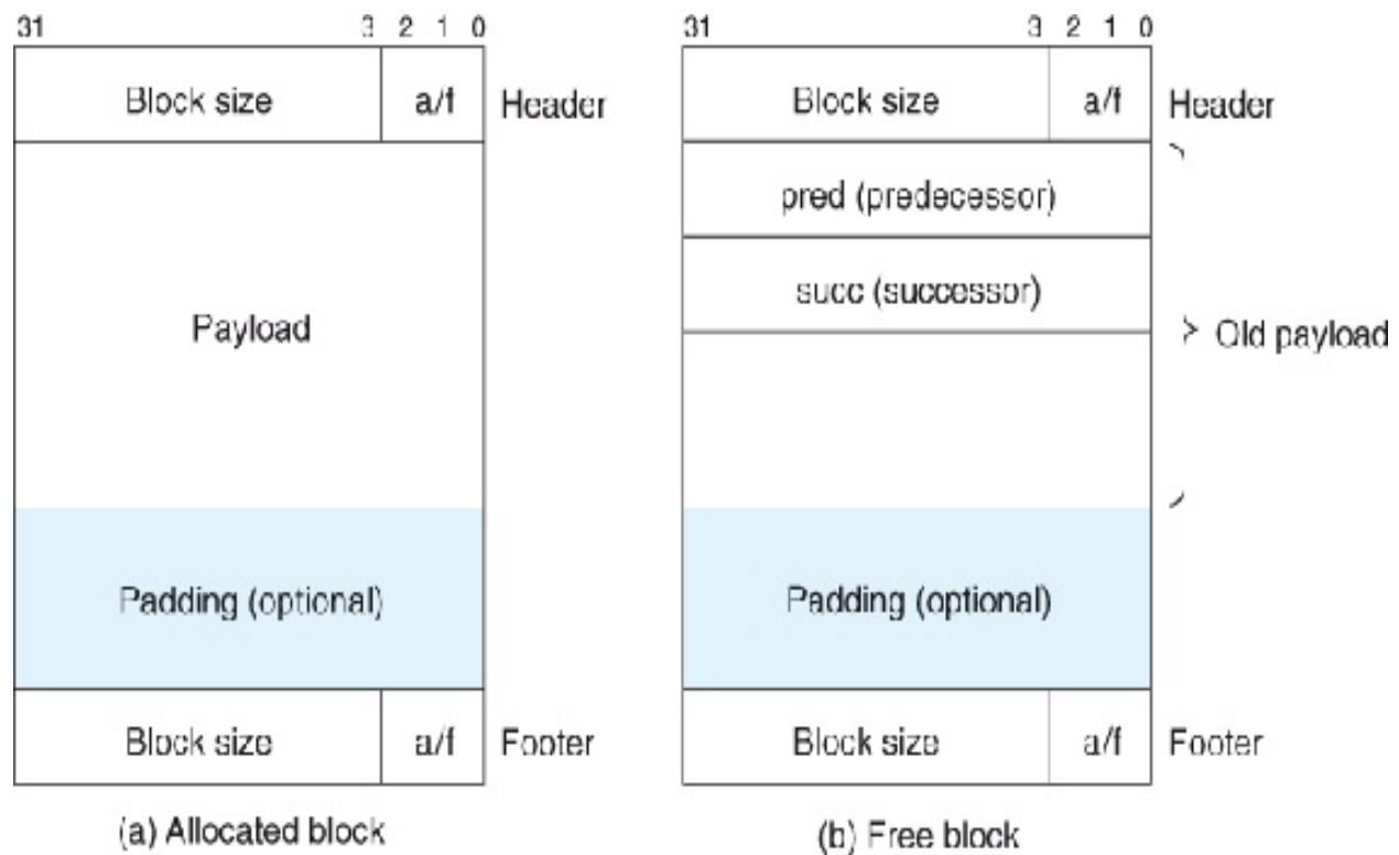
Figure 9.48 Format of heap blocks that use doubly linked free lists.
