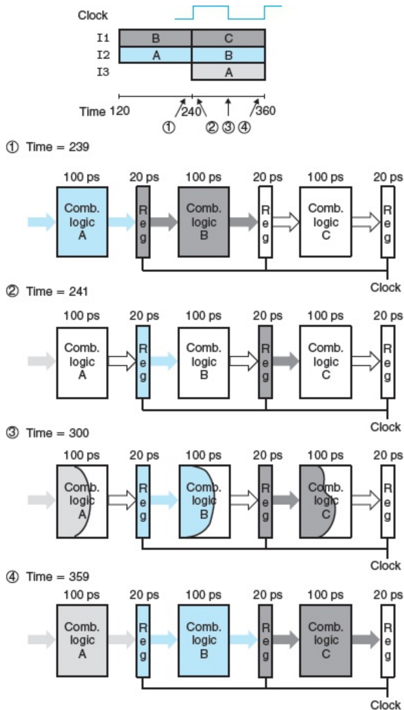
Figure 4.35 One clock cycle of pipeline operation.
