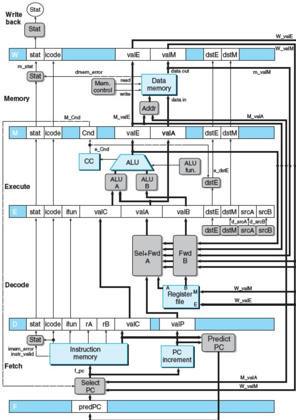
Figure 4.52 Hardware structure of PIPE, our final pipelined implementation.
