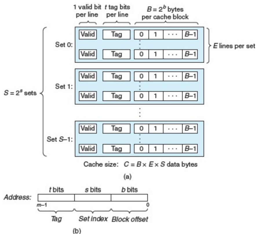
Figure 6.25 General organization of cache ( S , E , B , m ).
