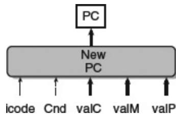
Figure 4.31 SEQ PC update stage.
