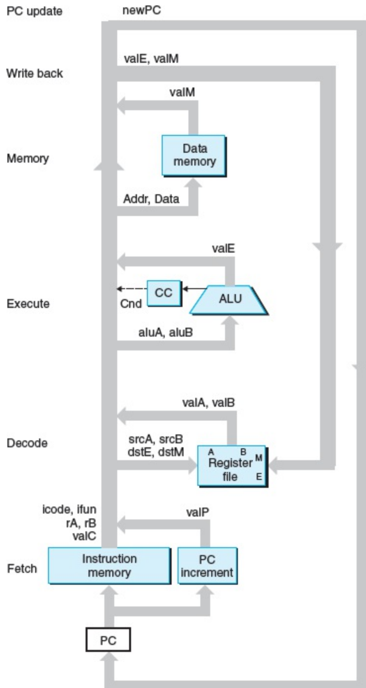
Figure 4.22 Abstract view of SEQ, a sequential implementation.
