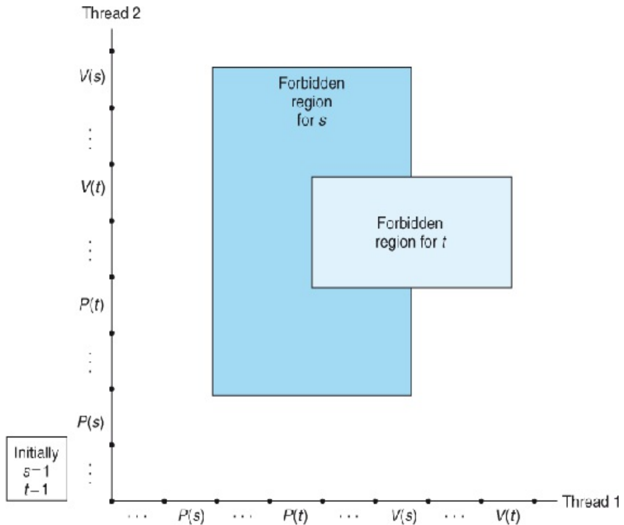
Figure 12.45 Progress graph for a deadlock-free program.
