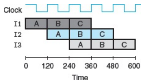
Figure 4.34 Three-stage pipeline timing.
