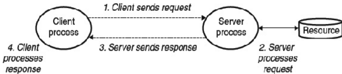
Figure 11.1 A client-server transaction.
