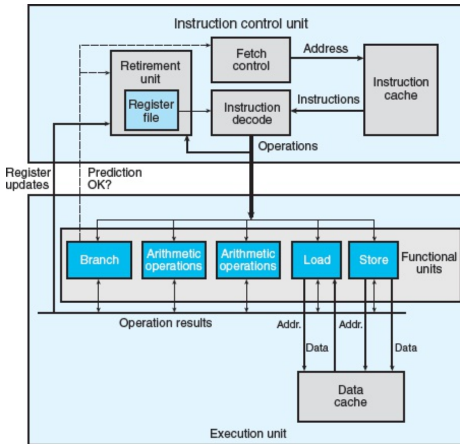
Figure 5.11 Block diagram of an out-of-order processor.
