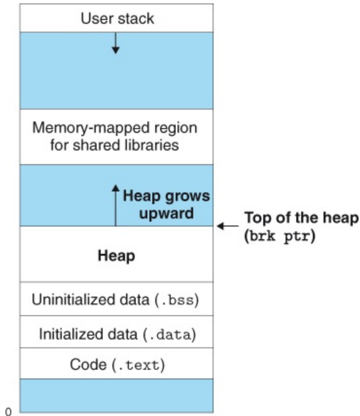
Figure 9.33 The heap.
