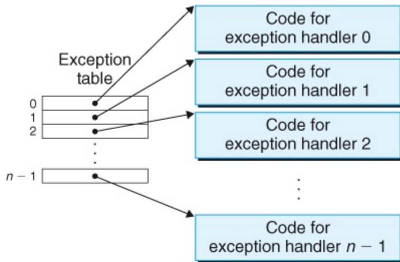
Figure 8.2 Exception table.
