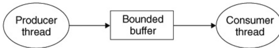
Figure 12.23 Producer-consumer problem.
