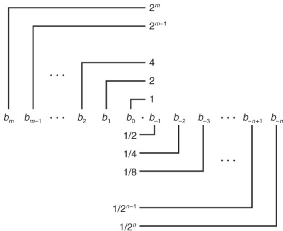
Figure 2.31 Fractional binary representation.
