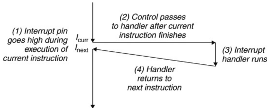
Figure 8.5 Interrupt handling.
