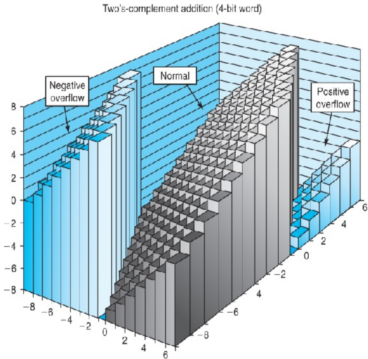
Figure 2.26 Two's-complement addition.
