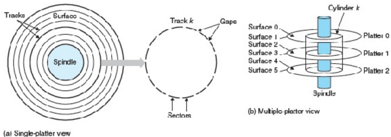
Figure 6.9 Disk geometry.
