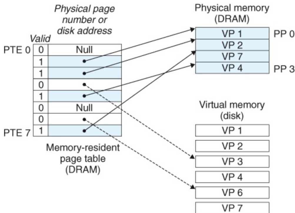
Figure 9.4 Page table.
