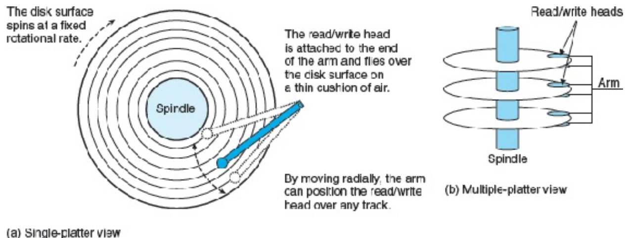
Figure 6.10 Disk dynamics.
