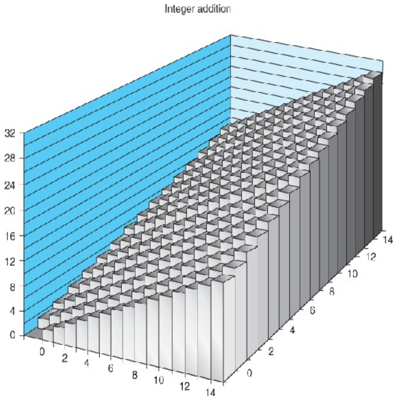
Figure 2.21 Integer addition.
