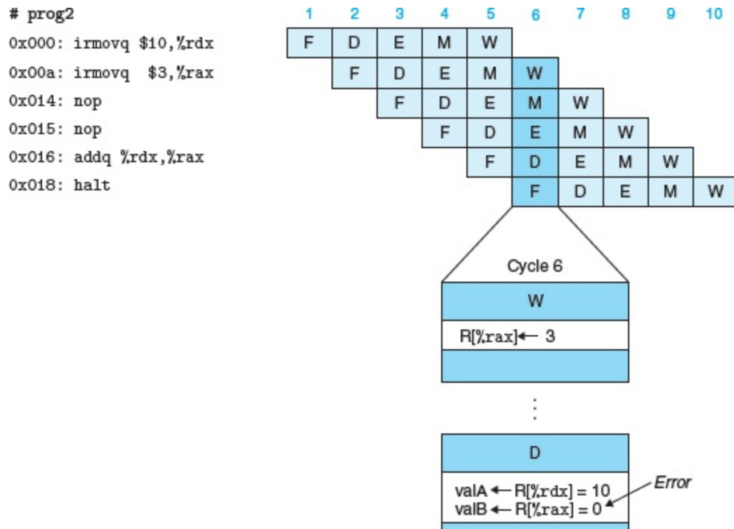
Figure 4.44 Pipelined execution of prog2 without special pipeline control.
