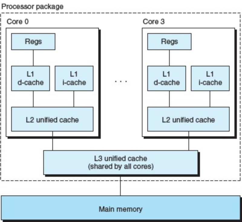
Figure 6.38 Intel Core i7 cache hierarchy.
