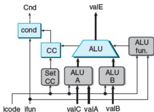
Figure 4.29 SEQ execute stage.
