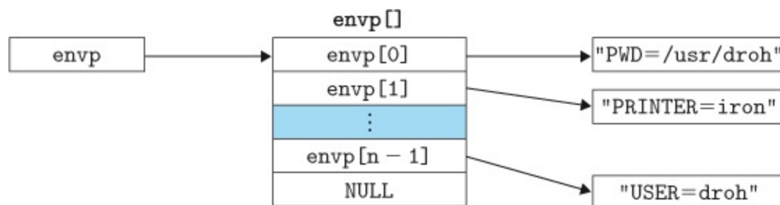
Figure 8.21 Organization of an environment variable list.
