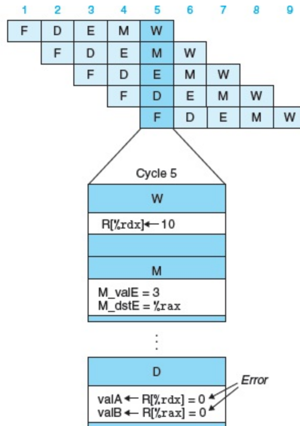
Figure 4.45 Pipelined execution of prog3 without special pipeline control.
