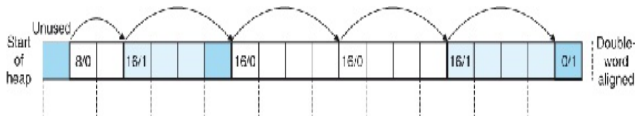
Figure 9.38 An example of false fragmentation.
