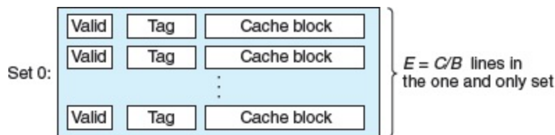
Figure 6.35 Fully associative cache ( E = C/B ).
