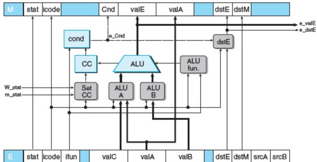
Figure 4.60 PIPE execute stage logic.
