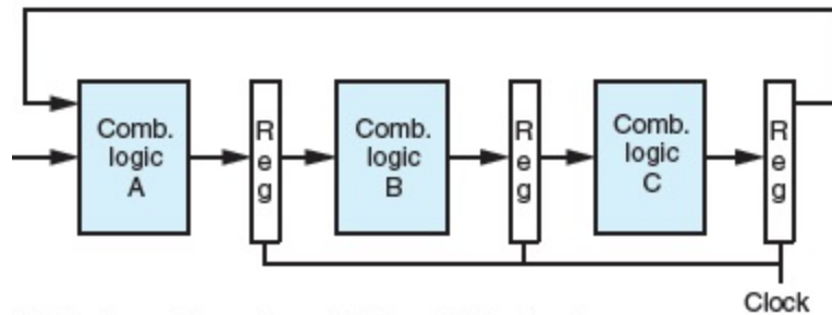
(c) Hardware: Three-stage pipeline with feedback
