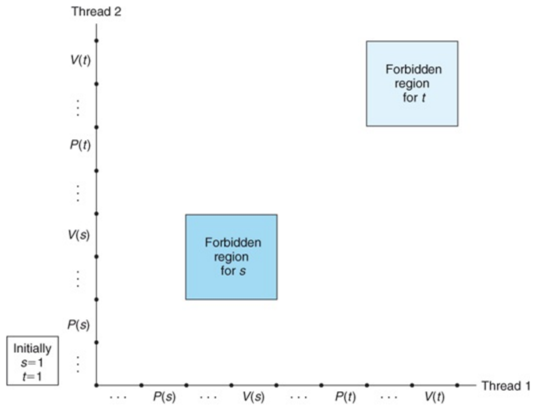
Figure 12.49 Progress graph for the corrected deadlock-free program.
