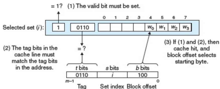
Figure 6.29 Line matching and word selection in a direct-mapped cache.
