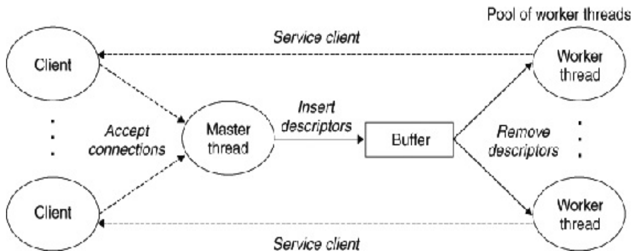
Figure 12.27 Organization of a prethreaded concurrent server.
