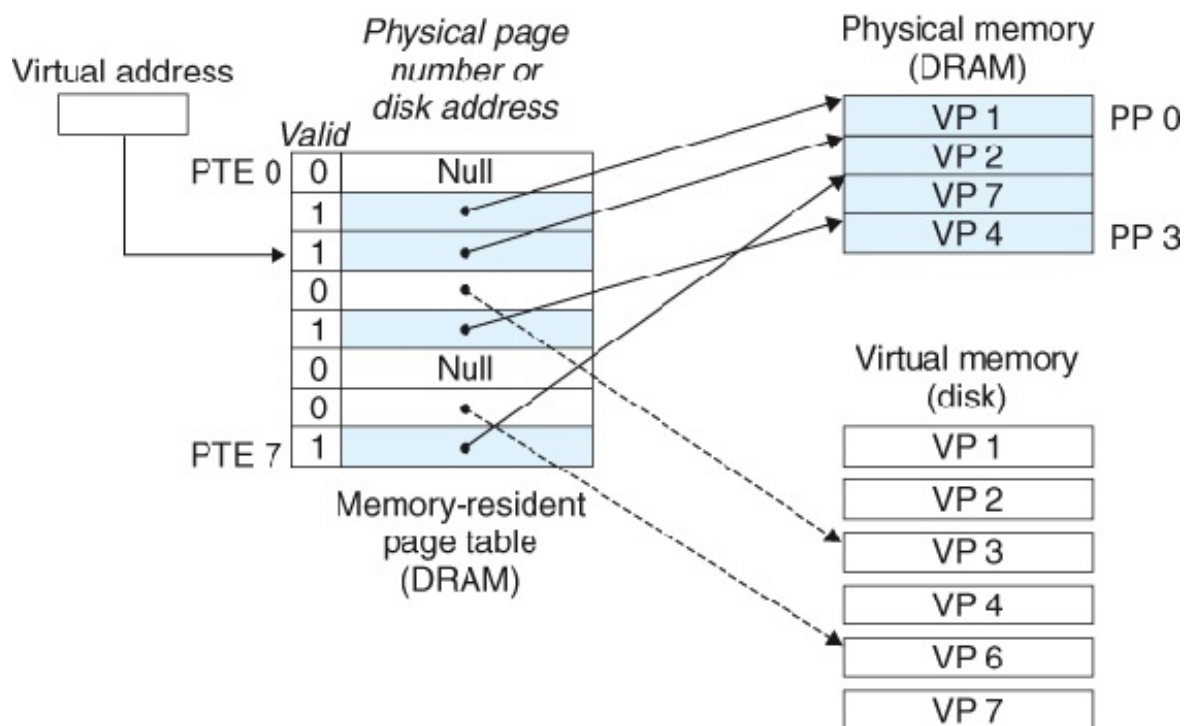
Figure 9.5 VM page hit.
