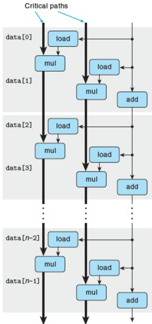
Figure 5.24 Data-flow representation of combine6 operating on a vector of length n .
