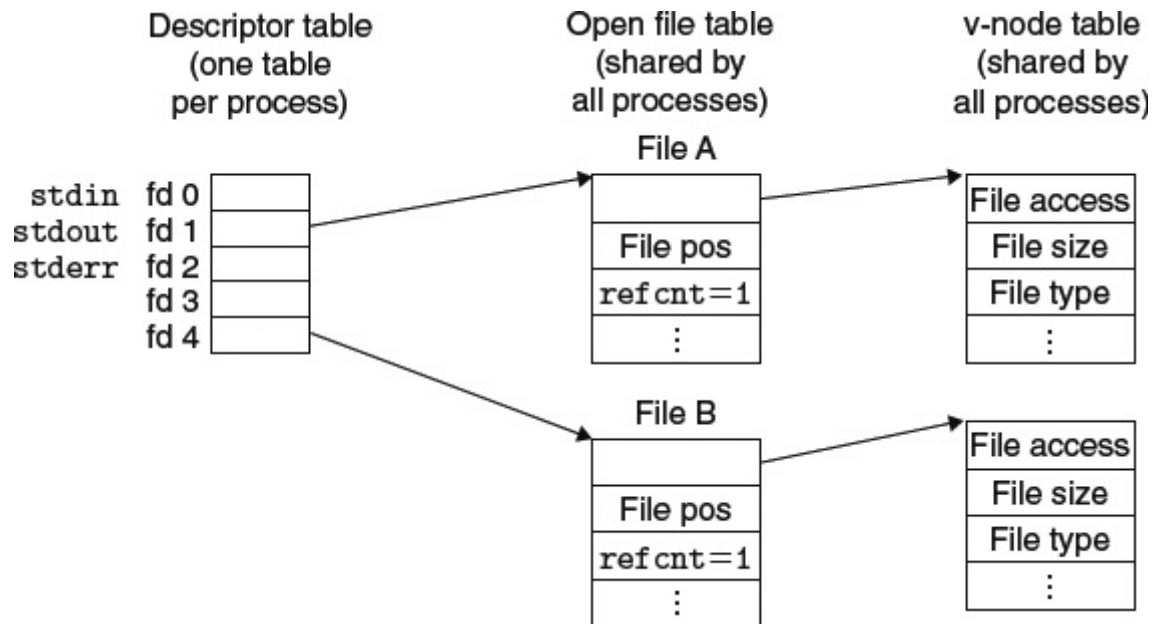
Figure 10.12 Typical kernel data structures for open files.
