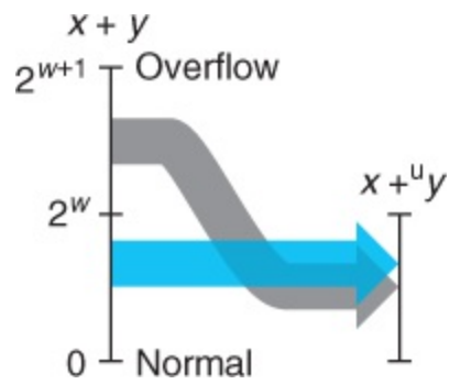
Figure 2.22 Relation between integer addition and unsigned addition.
