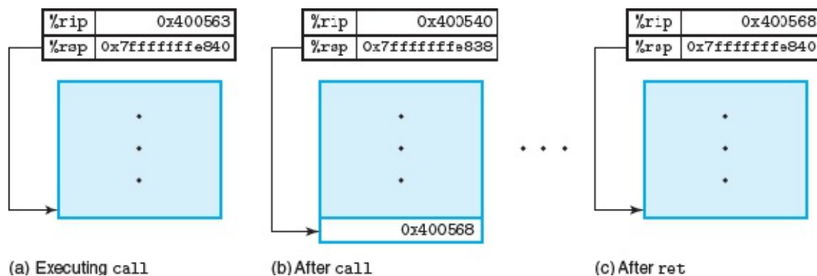
Figure 3.26 Illustration of call and ret functions.
