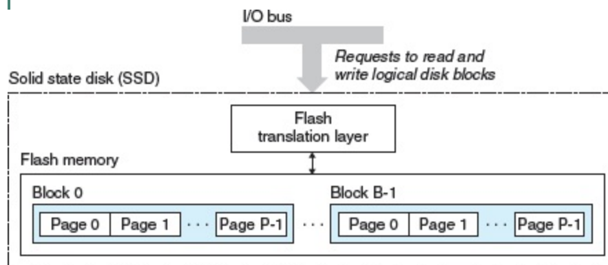
Figure 6.13 Solid state disk (SSD).
