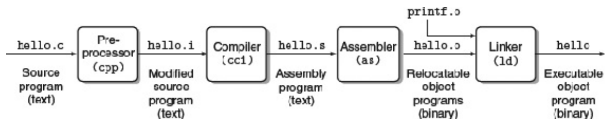
Figure 1.3 The compilation system.
