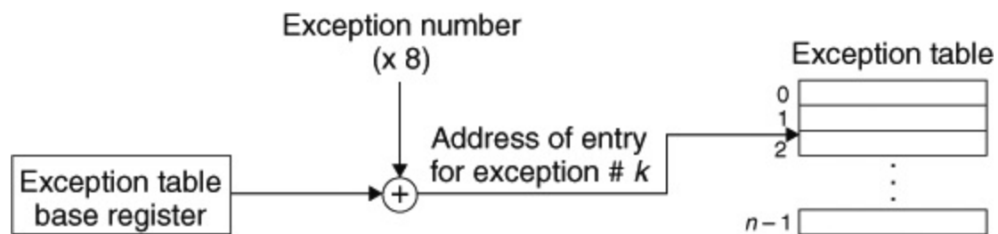
Figure 8.3 Generating the address of an exception handler.
