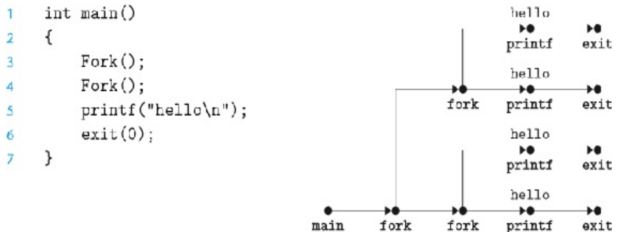
Figure 8.17 Process graph for a nested fork .
