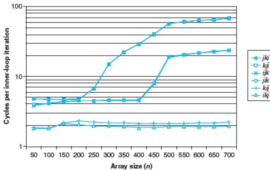
Figure 6.46 Core i7 matrix multiply performance.
