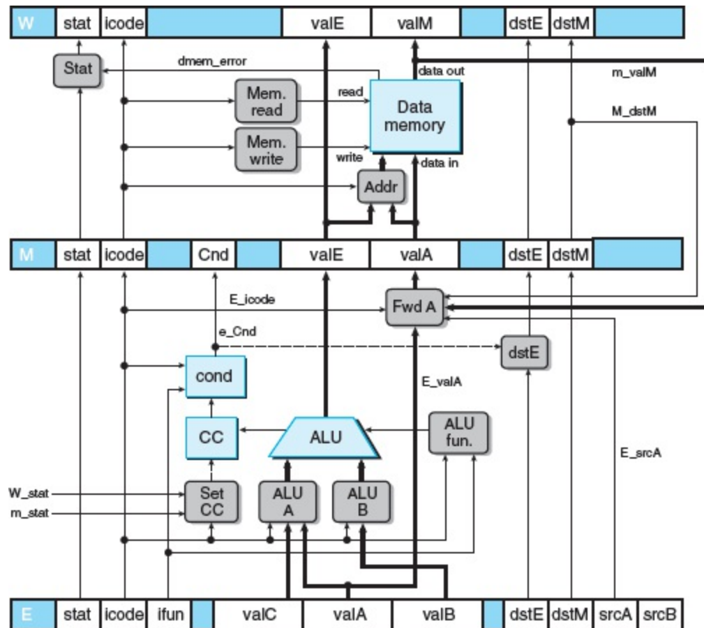
Figure 4.70 Execute and memory stages capable of load forwarding.
