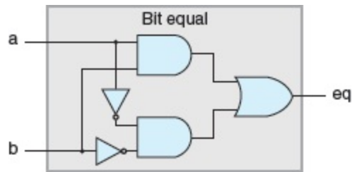
Figure 4.10 Combinational circuit to test for bit equality.
