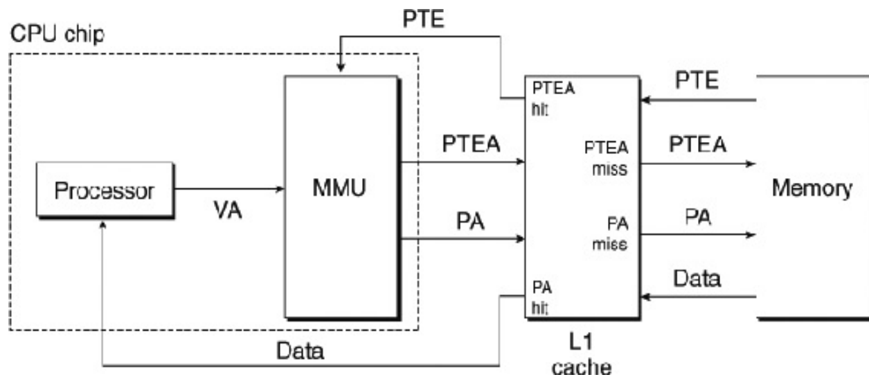
Figure 9.14 Integrating VM with a physically addressed cache.
