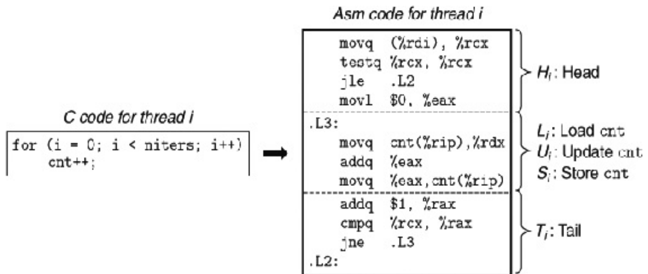
Figure 12.17 Assembly code for the counter loop (lines 40–41) in badcnt.c .
