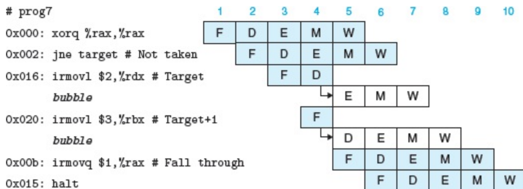
Figure 4.56 Processing mispredicted branch instructions.
