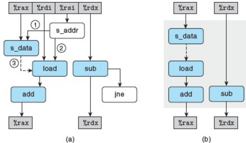
Figure 5.36 Abstracting the operations for write_read .
