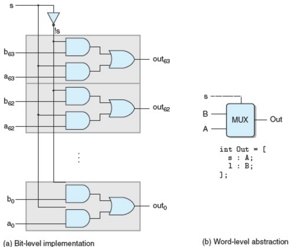
Figure 4.13 Word-level multiplexor circuit.
