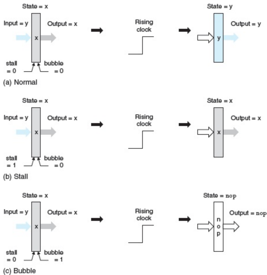
Figure 4.65 Additional pipeline register operations,
