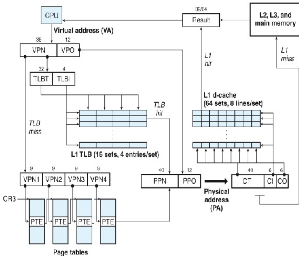
Figure 9.22 Summary of Core i7 address translation.
