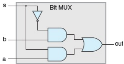
Figure 4.11 Single-bit multiplexor circuit.
