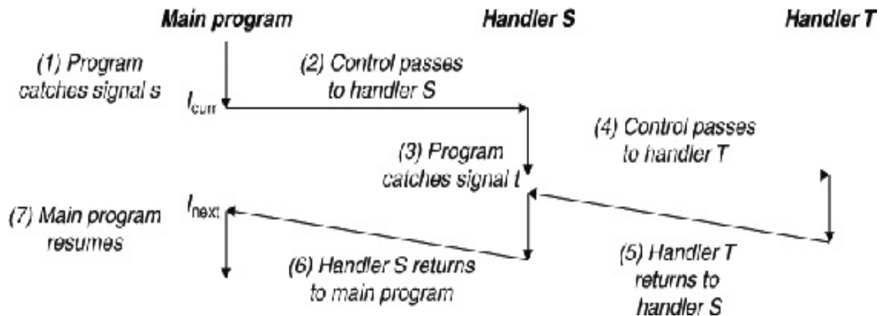
Figure 8.31 Handlers can be interrupted by other handlers.
