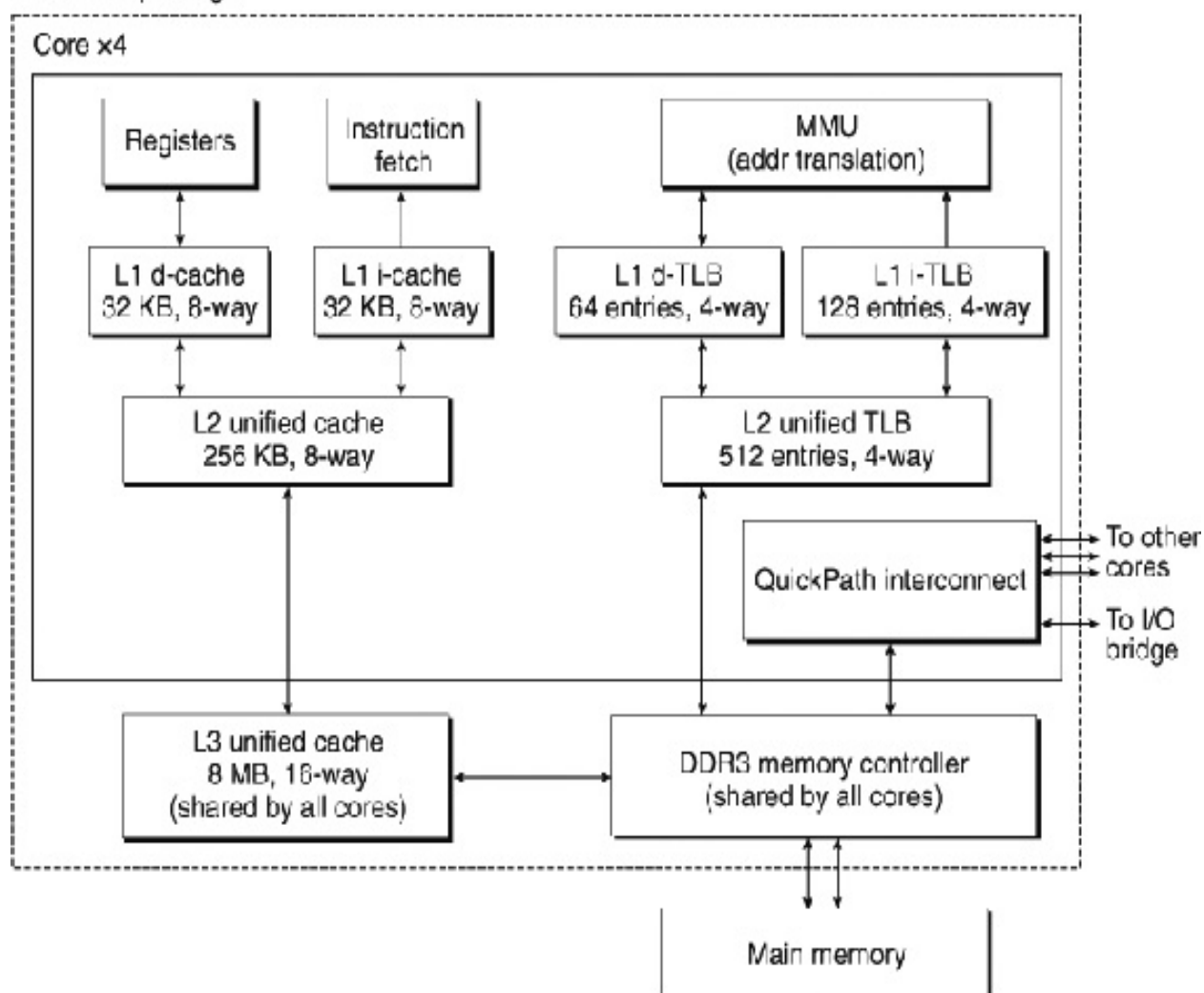
Figure 9.21 The Core i7 memory system.
