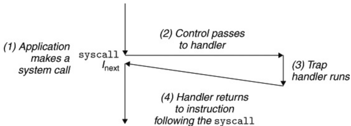
Figure 8.6 Trap handling.
