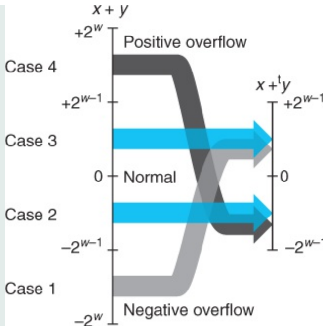
Figure 2.24 Relation between integer and two's-complement addition.
