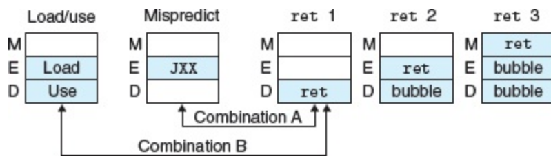
Figure 4.67 Pipeline states for special control conditions.
