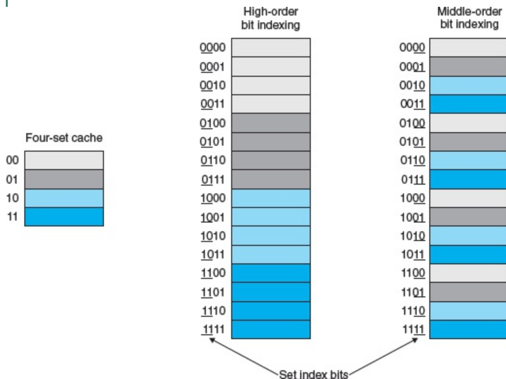
Figure 6.31 Why caches index with the middle bits.
