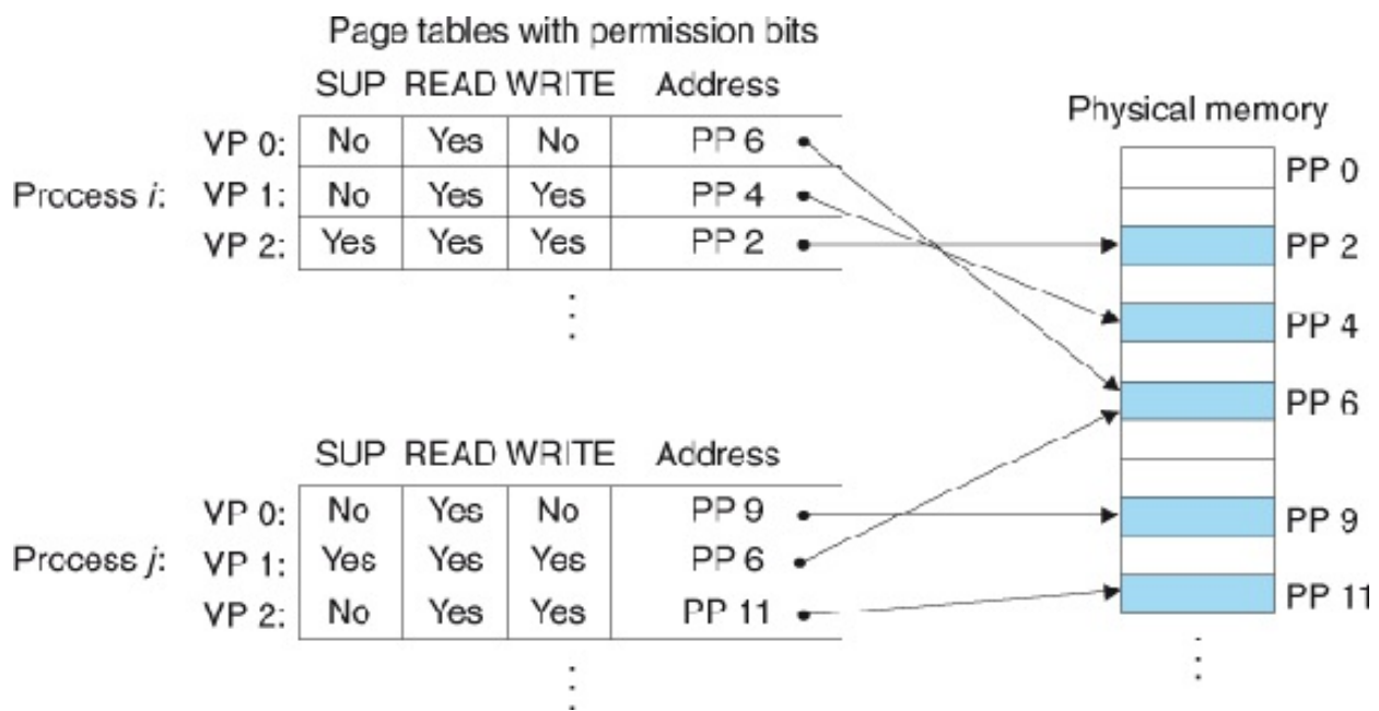
Figure 9.10 Using VM to provide page-level memory protection.
