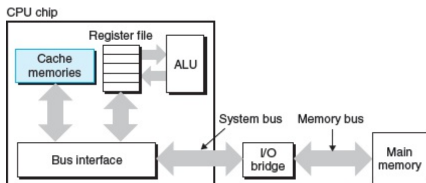
Figure 6.24 Typical bus structure for cache memories.
