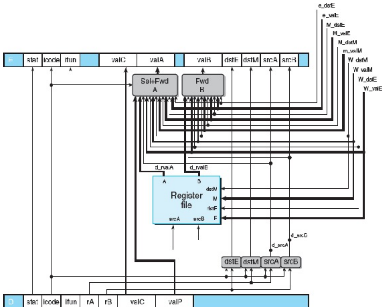
Figure 4.58 PIPE decode and write-back stage logic.
