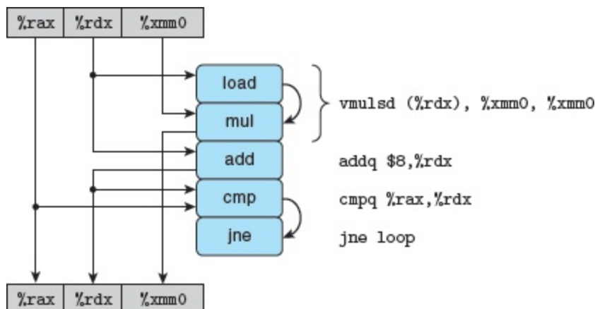
Figure 5.13 Graphical representation of inner-loop code for combine4
