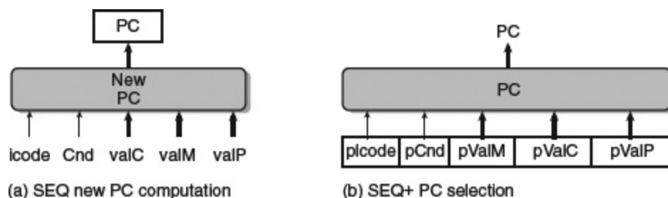
Figure 4.39 Shifting the timing of the PC computation.
