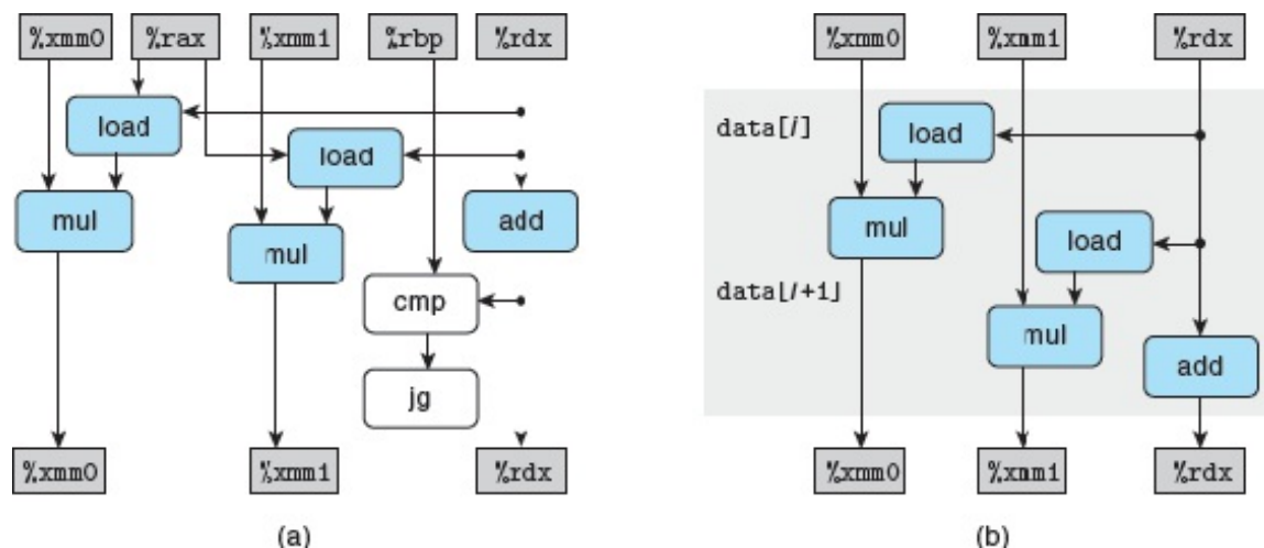
Figure 5.23 Abstracting combine6 operations as a data-flow graph.
