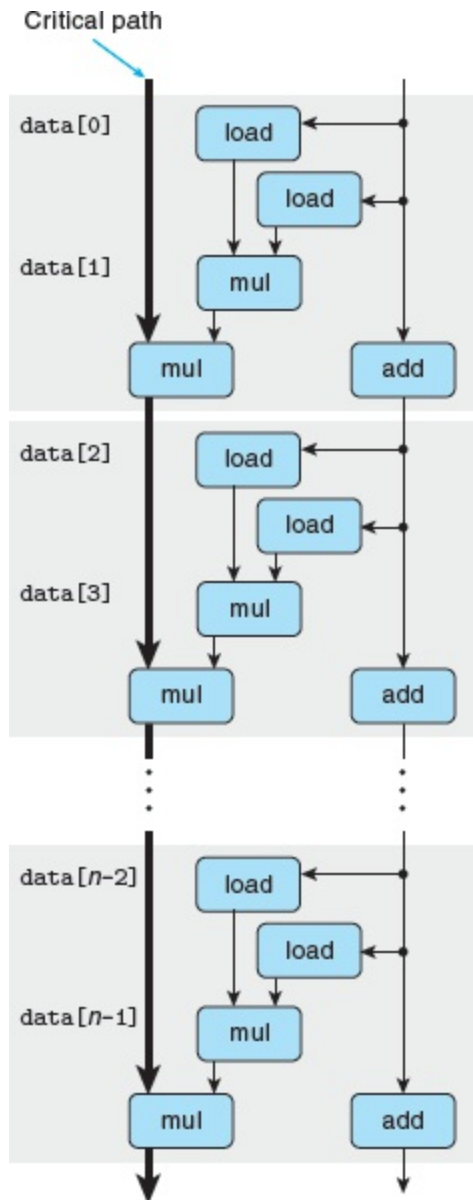
Figure 5.29 Data-flow representation of combine7 operating on a vector of length n .
