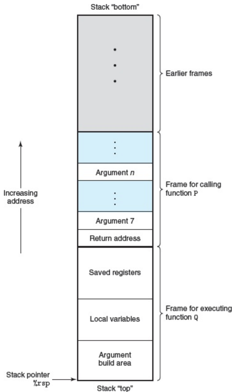
Figure 3.25 General stack frame structure.
