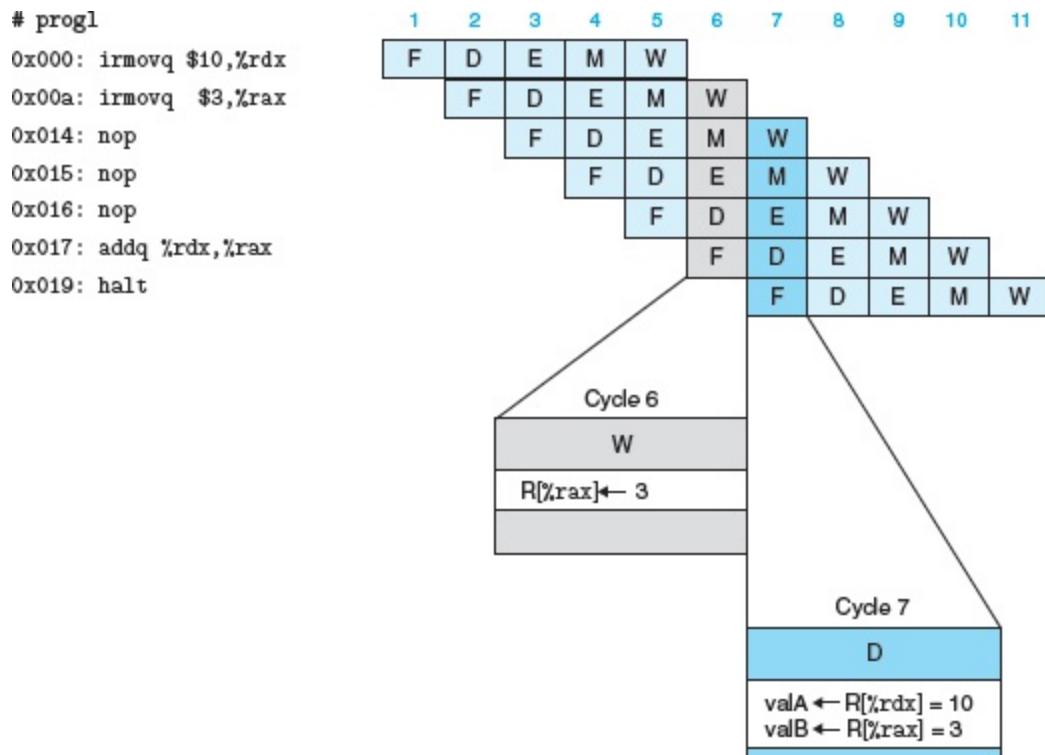
Figure 4.43 Pipelined execution of prog1 without special pipeline control.
