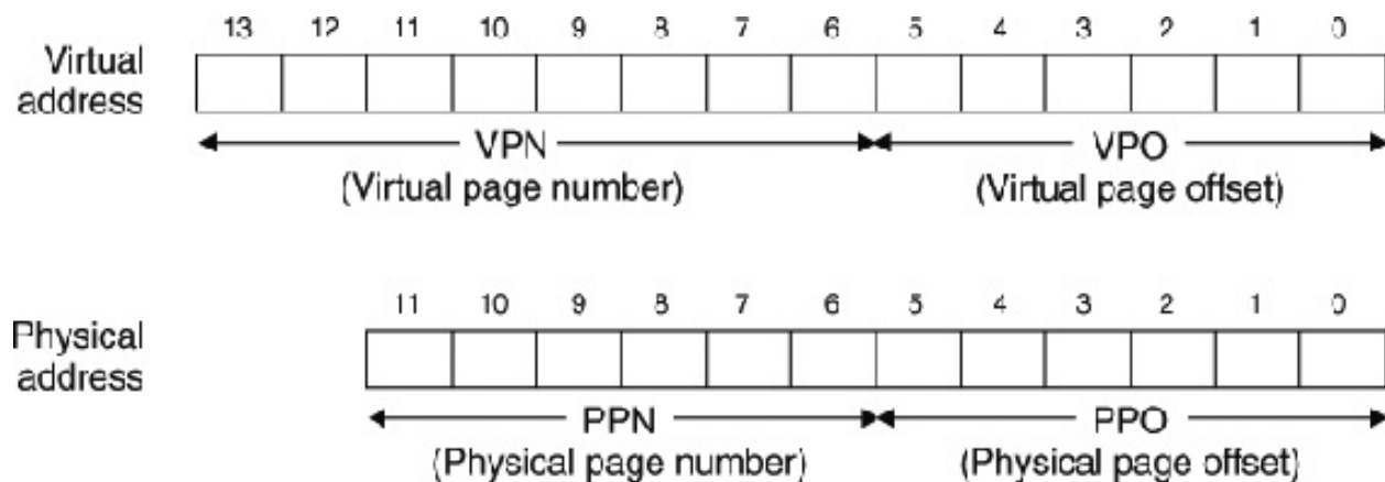
Figure 9.19 Addressing for small memory system.
