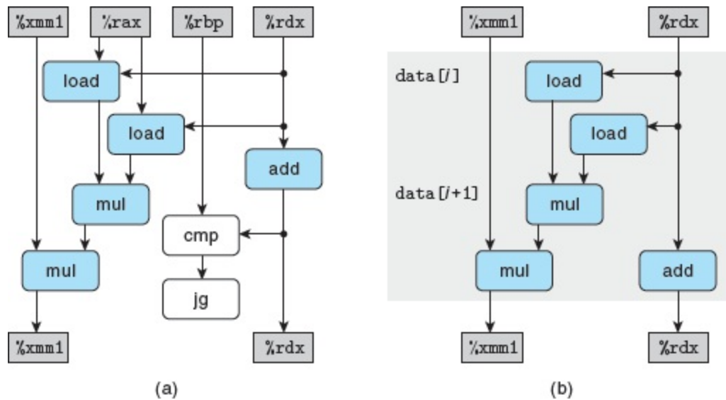
Figure 5.28 Abstracting combine7 operations as a data-flow graph.
