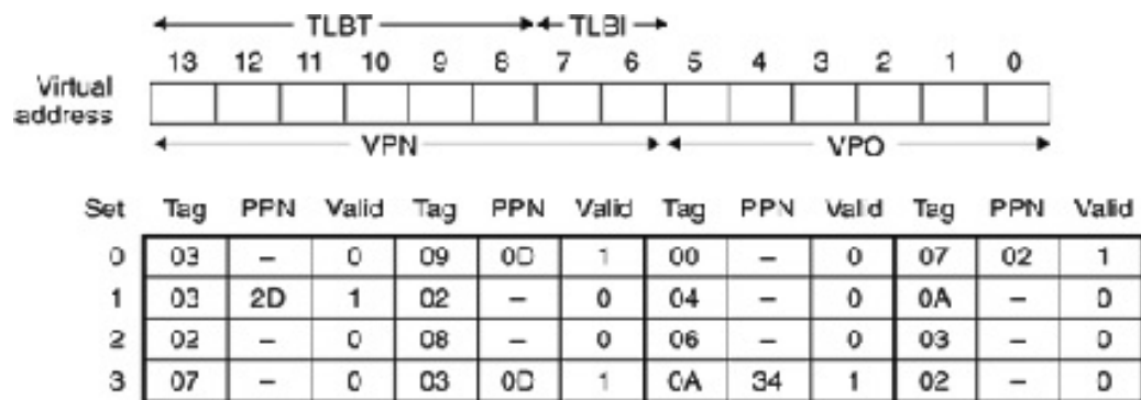
(a) TLB: 4 sets, 16 entries, 4-way set associative
