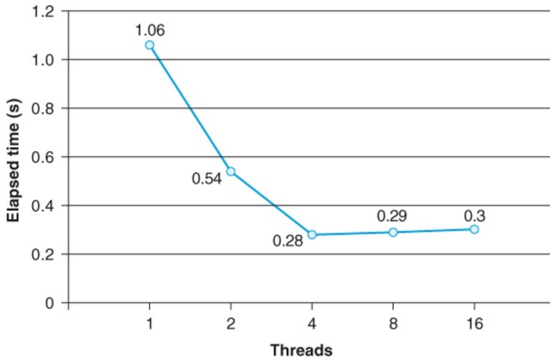
Figure 12.35 Performance of psum-local (Figure 12.34 □ ). Summing a sequence of 2^{31} elements using four processor cores.
