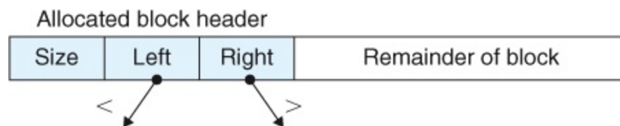
Figure 9.53 Left and right pointers in a balanced tree of allocated blocks.
