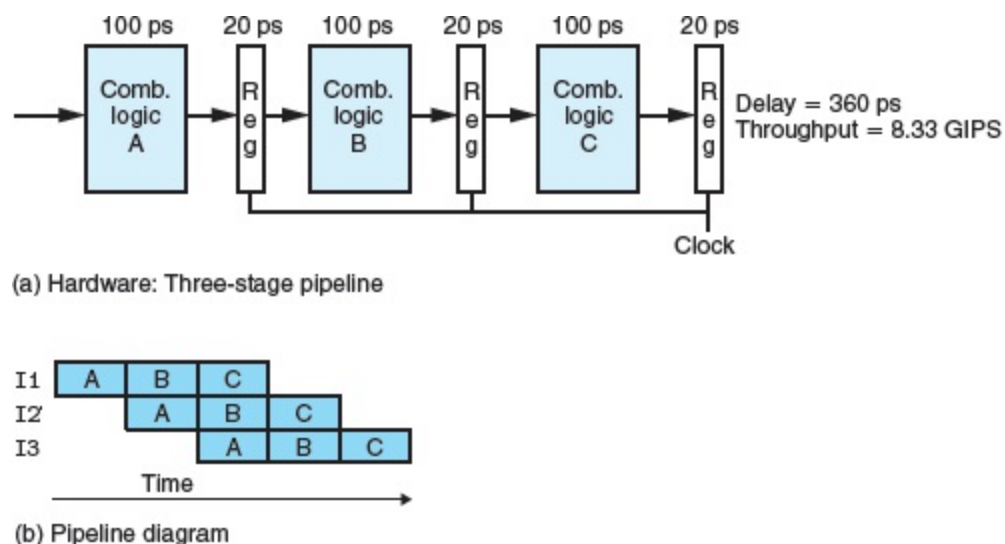
Figure 4.33 Three-stage pipelined computation hardware.
