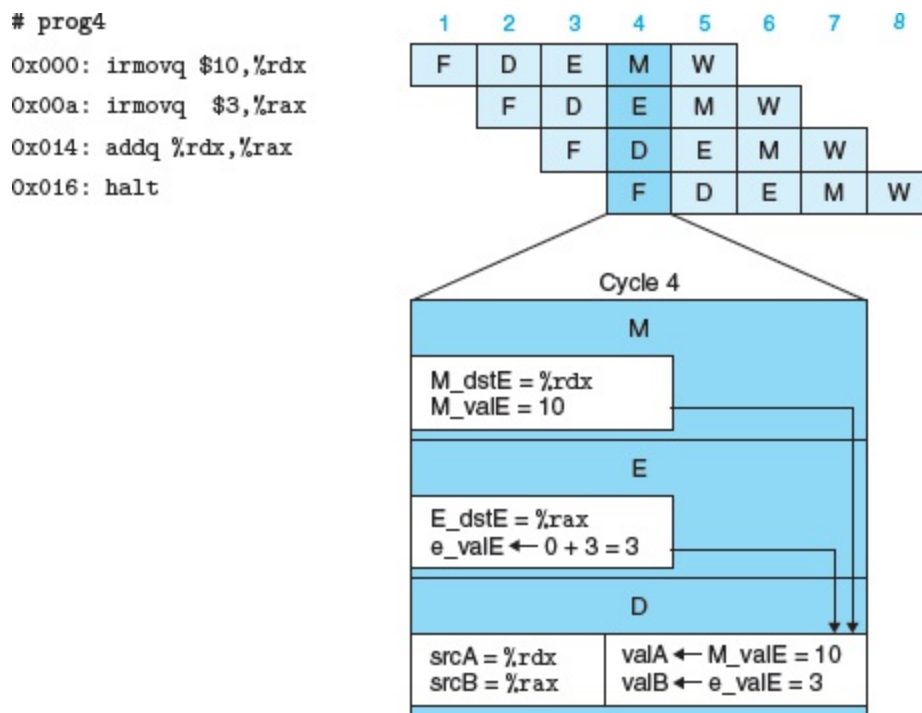
Figure 4.51 Pipelined execution of prog4 using forwarding.
