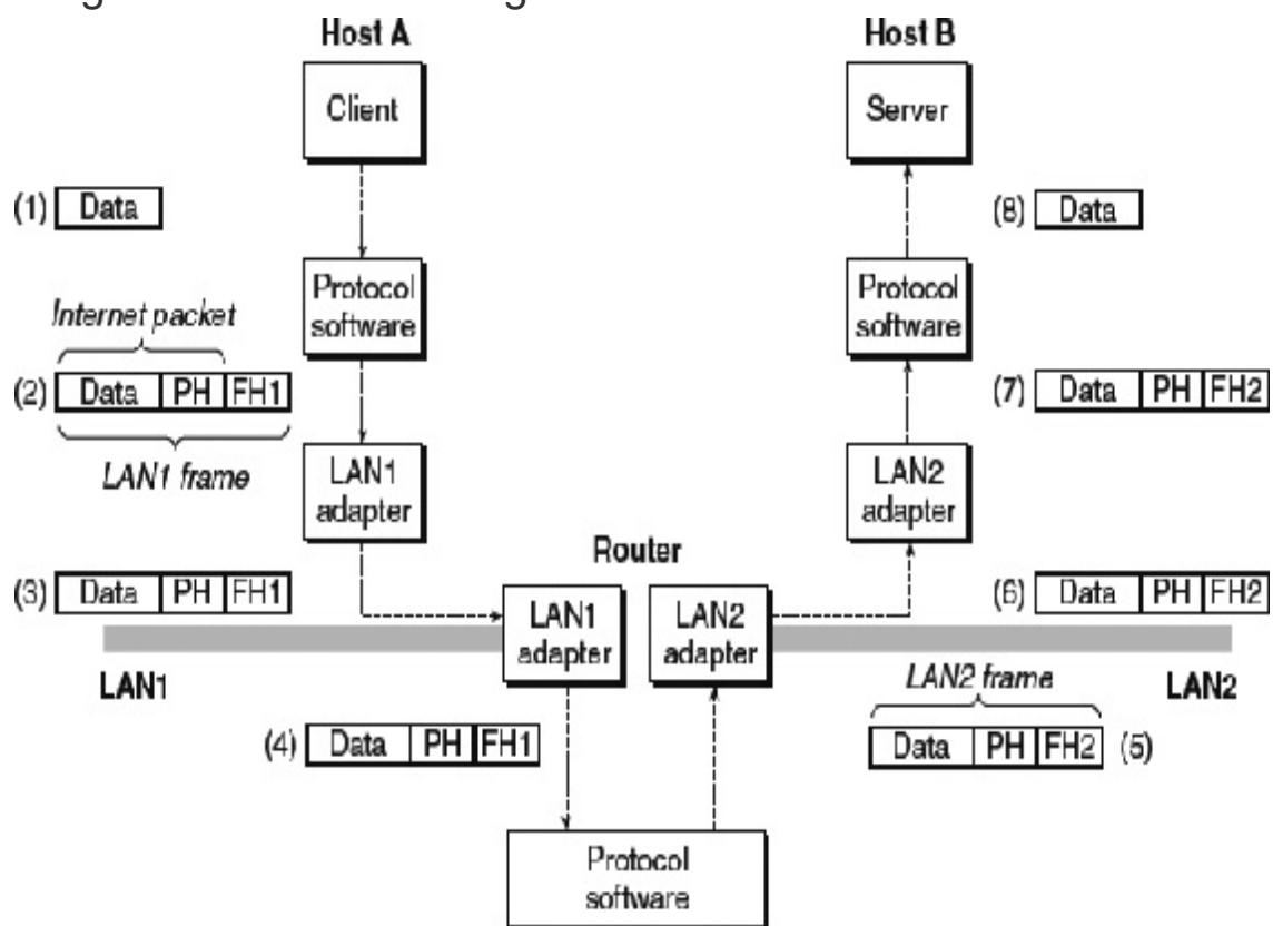
Figure 11.7 How data travel from one host to another on an internet.
