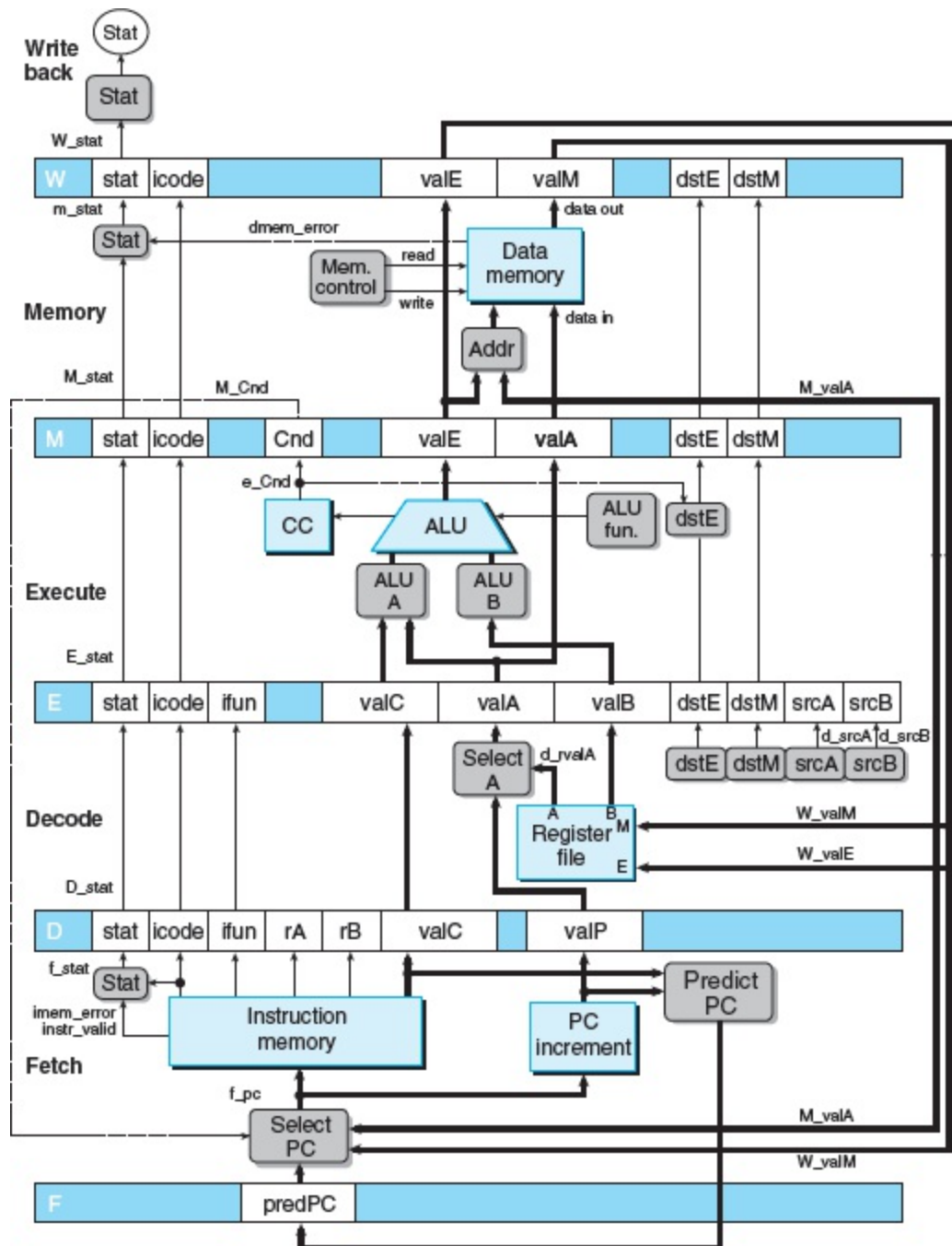
Figure 4.41 Hardware structure of PIPE—, an initial pipelined implementation.
