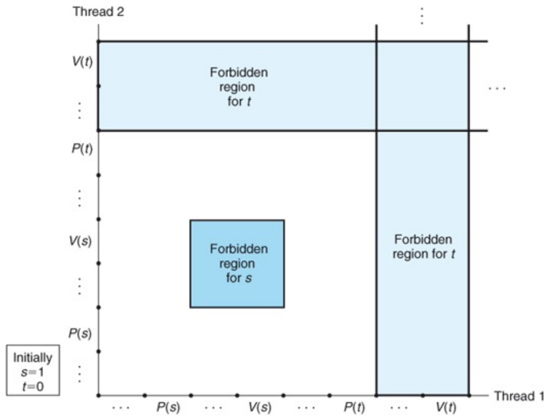
Figure 12.48 Progress graph for a program that deadlocks.
