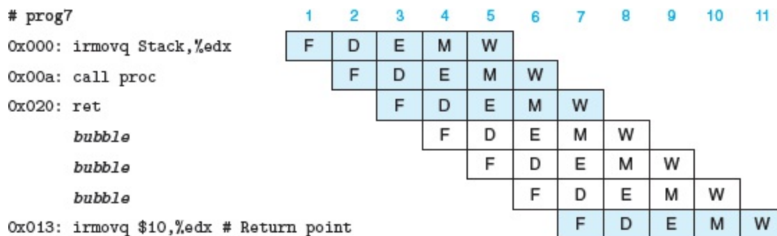
Figure 4.55 Simplified view of ret instruction processing.
