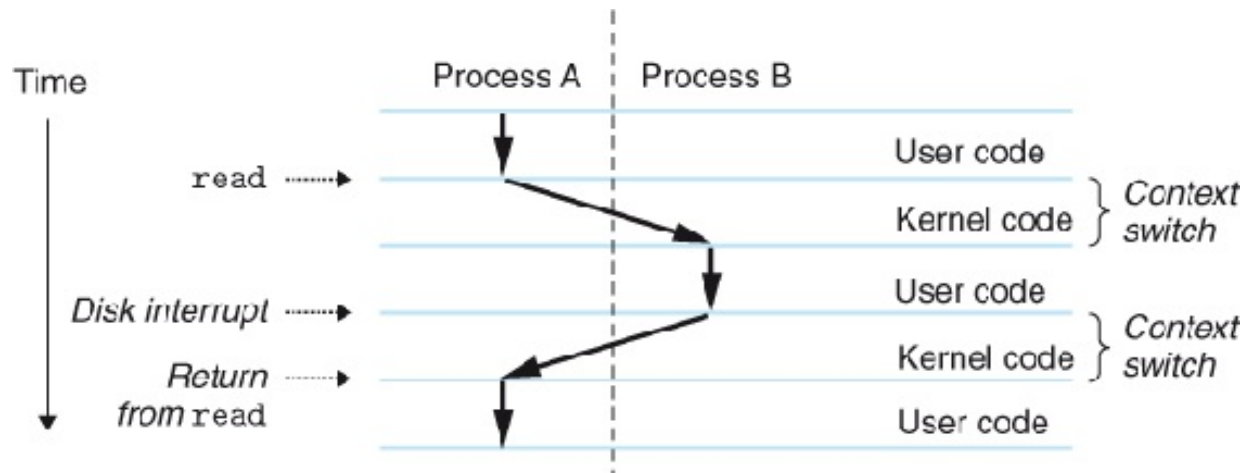
Figure 8.14 Anatomy of a process context switch.
