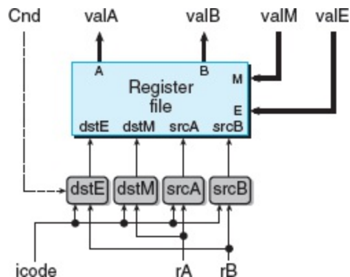
Figure 4.28 SEQ decode and write-back stage.
