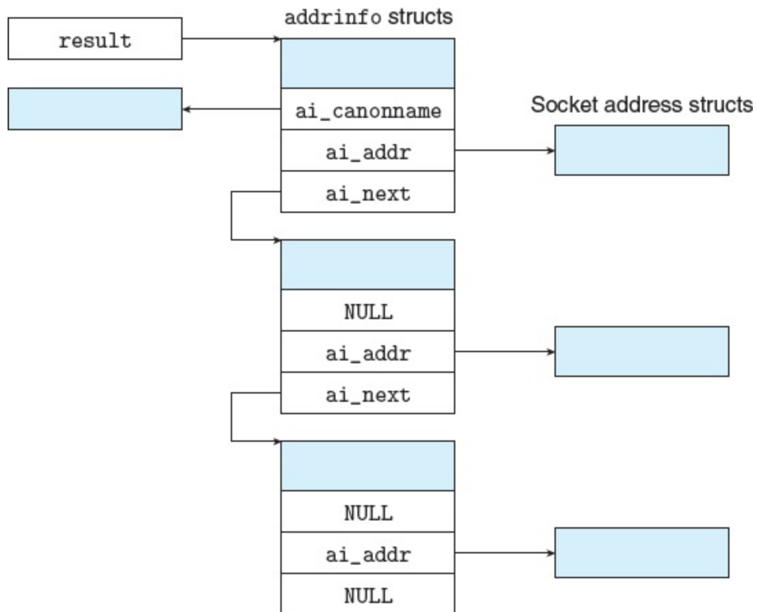
Figure 11.15 Data structure returned by getaddrinfo .
