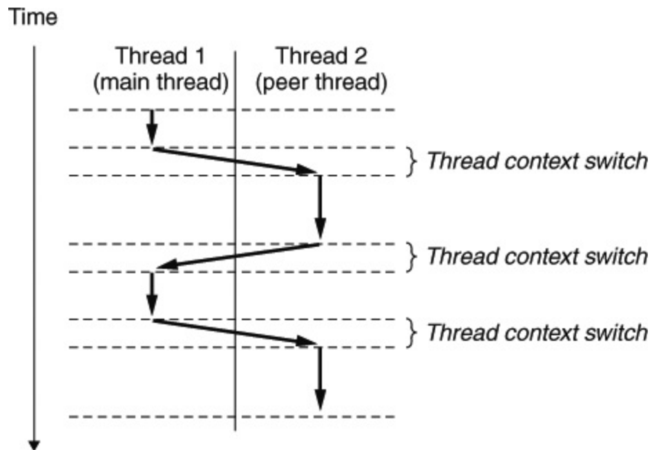
Figure 12.12 Concurrent thread execution.
