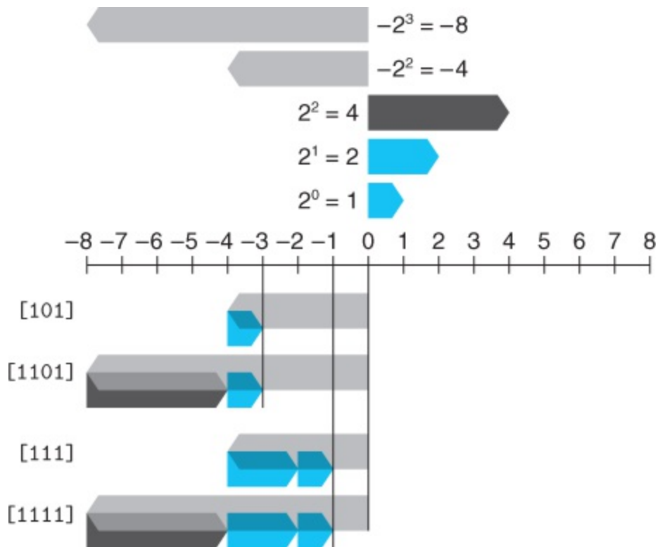
Figure 2.20 Examples of sign extension from w = 3 to w = 4 .
