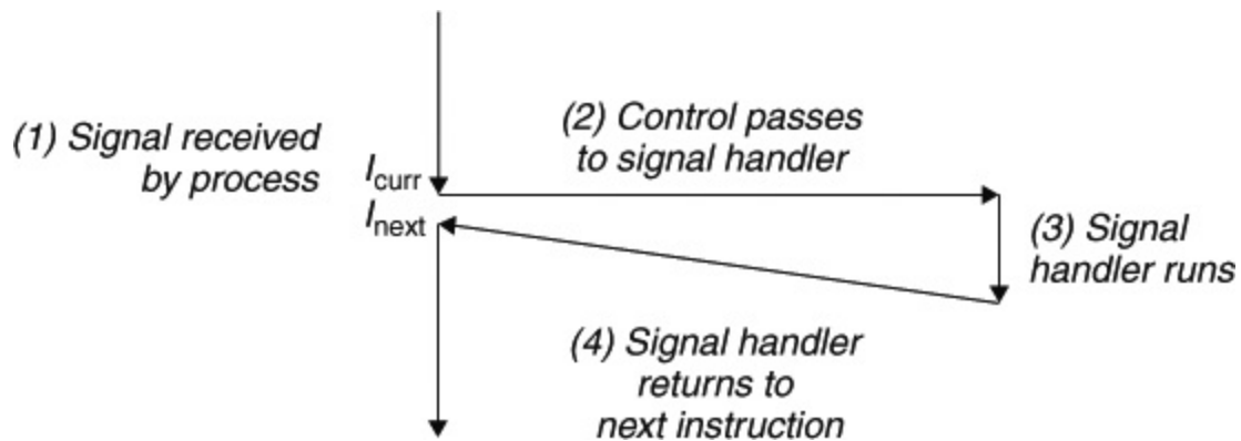
Figure 8.27 Signal handling.
