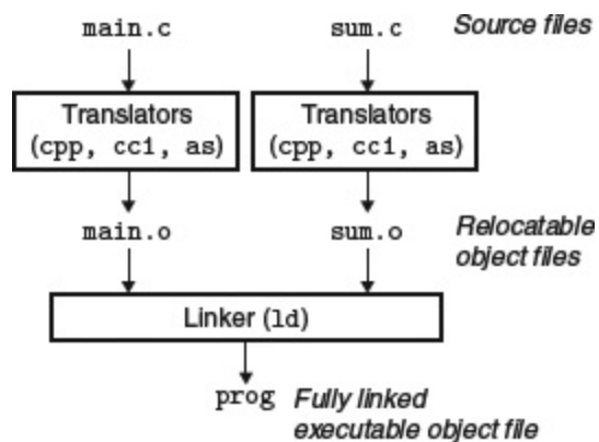
Figure 7.2 Static linking.
