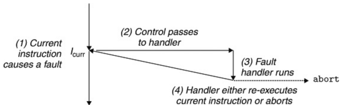
Figure 8.7 Fault handling.
