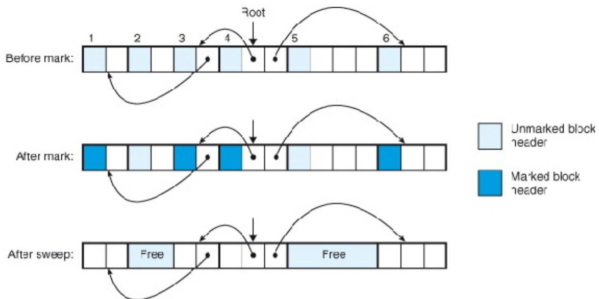
Figure 9.52 Mark&Sweep example.
