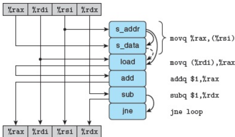
Figure 5.35 Graphical representation of inner-loop code for write_read .
