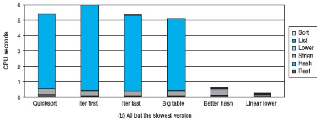
Figure 5.38 Profile results for different versions of bigram-frequency counting program.
