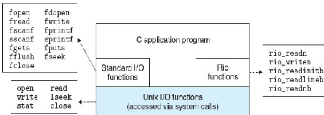
Figure 10.16 Relationship between Unix I/O, standard I/O, and RIo.
