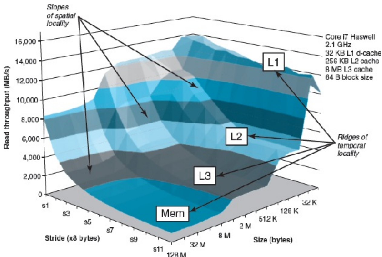
Figure 6.41 A memory mountain.
