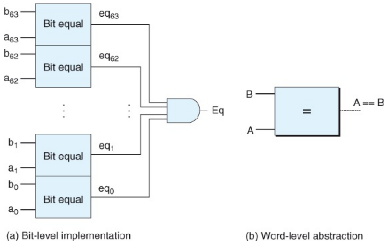
Figure 4.12 Word-level equality test circuit.
