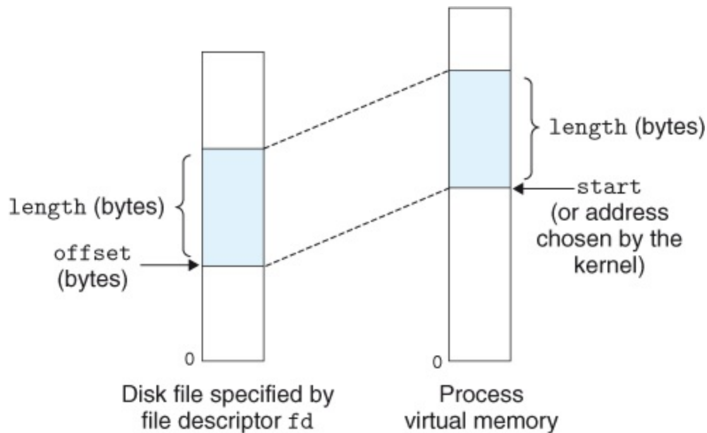
Figure 9.32 Visual interpretation of mmap arguments.
