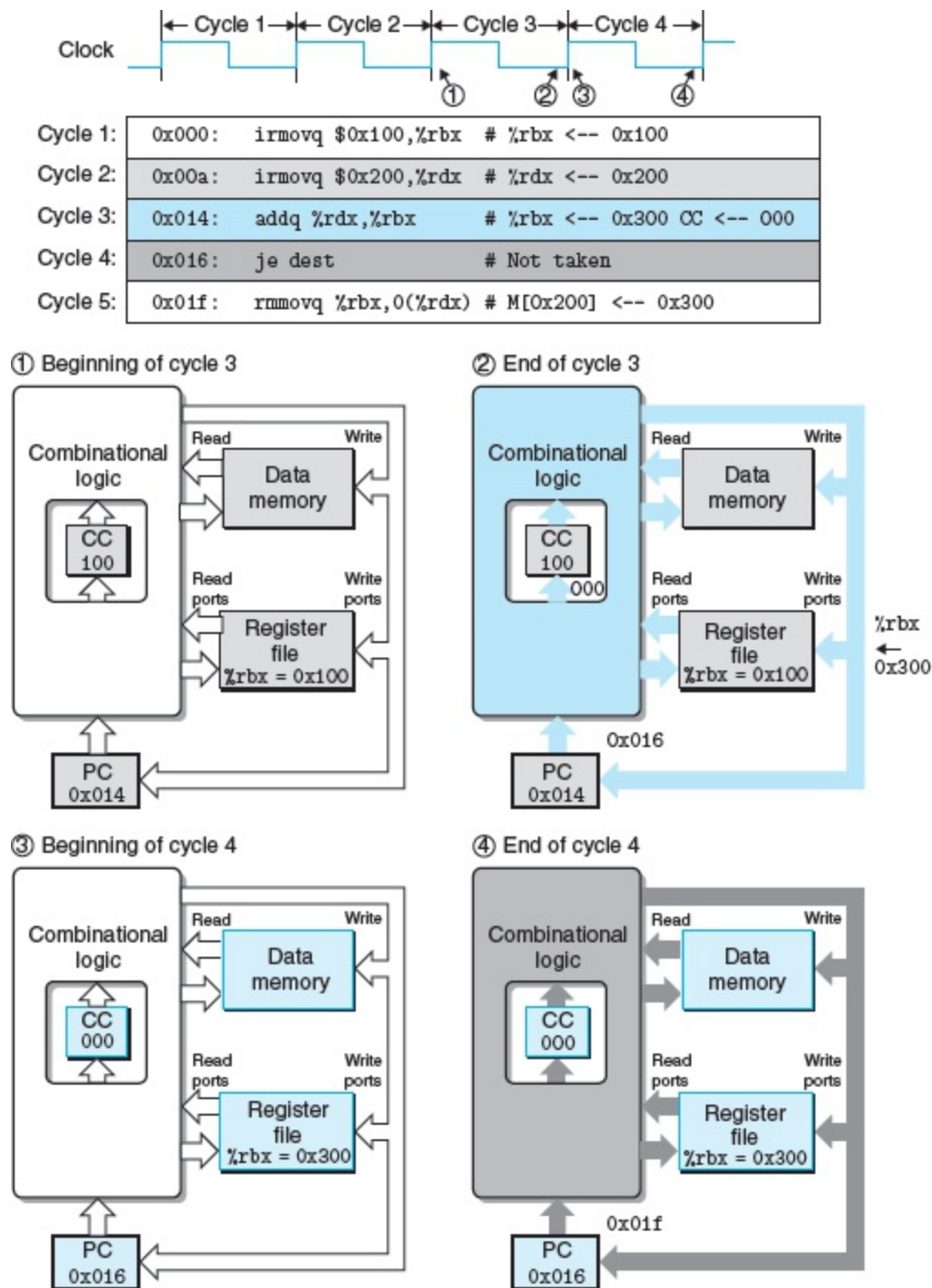
Figure 4.25 Tracing two cycles of execution by SEQ.
