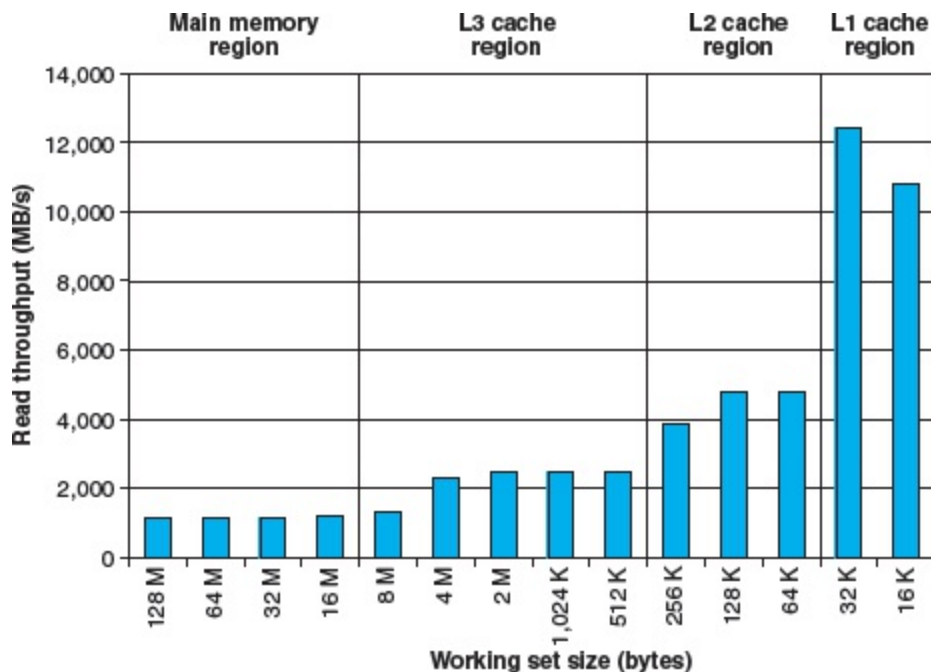
Figure 6.42 Ridges of temporal locality in the memory mountain.
