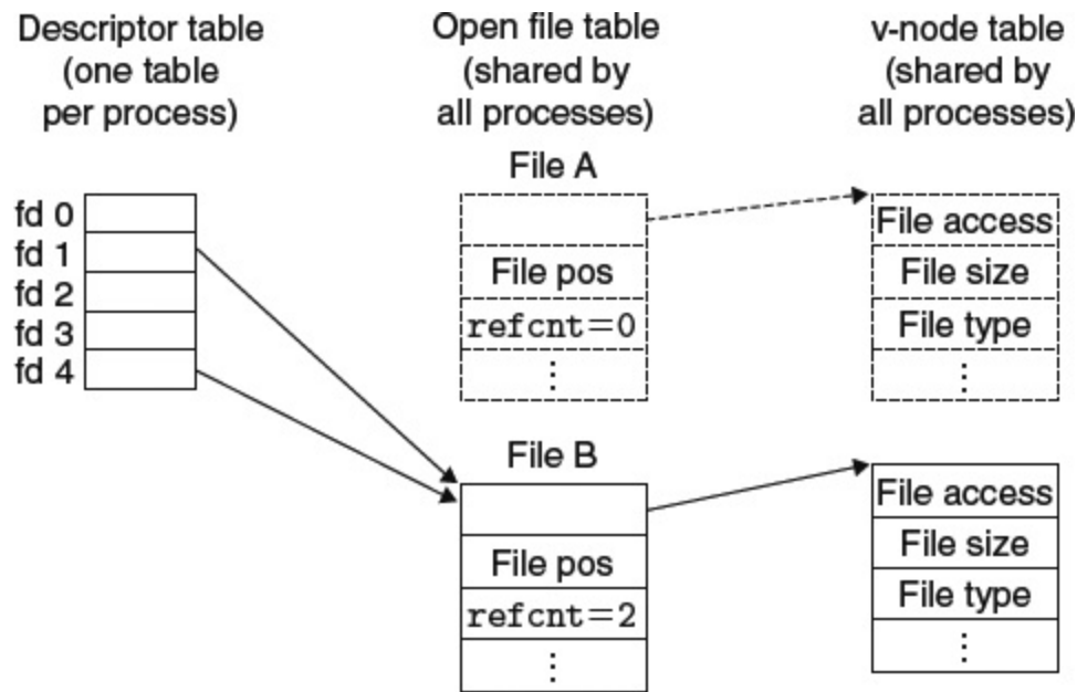
Figure 10.15 Kernel data structures after redirecting standard output by calling dup2(4, 1) .
