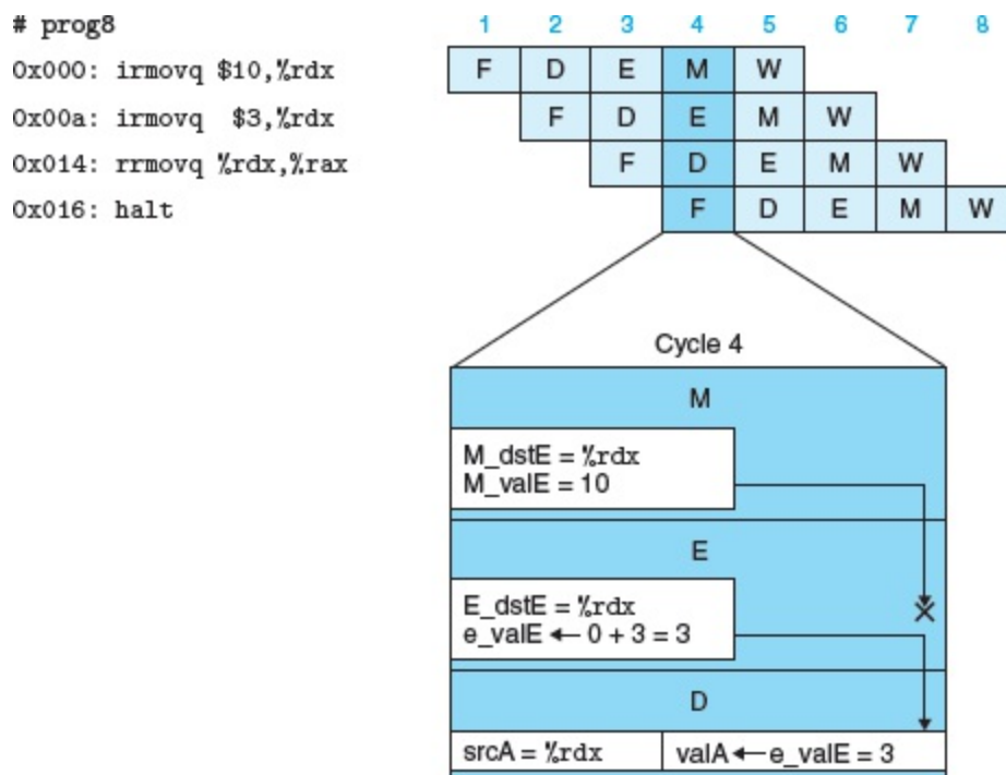
Figure 4.59 Demonstration of forwarding priority.
