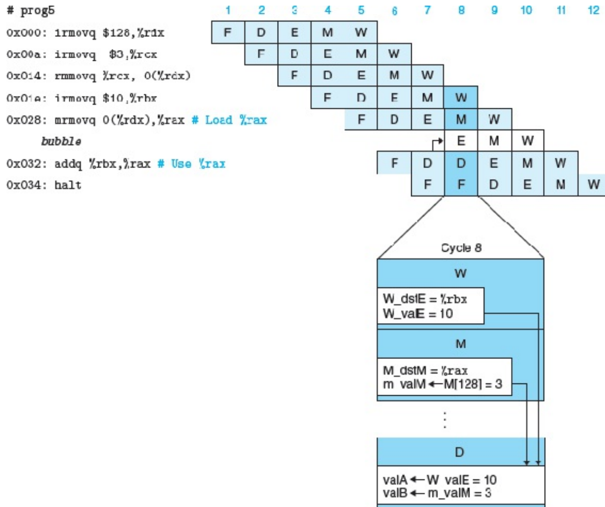
Figure 4.54 Handling a load/use hazard by stalling.
