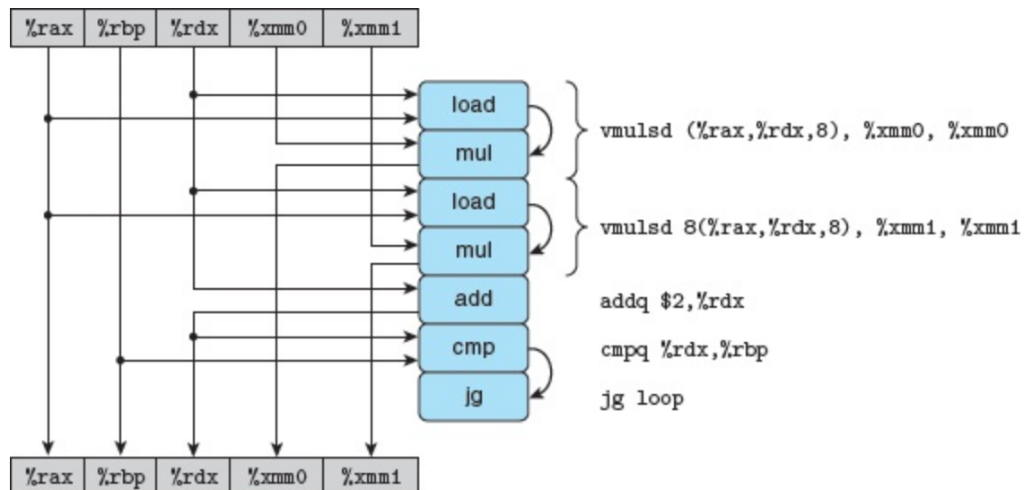
Figure 5.22 Graphical representation of inner-loop code for combine6 .
