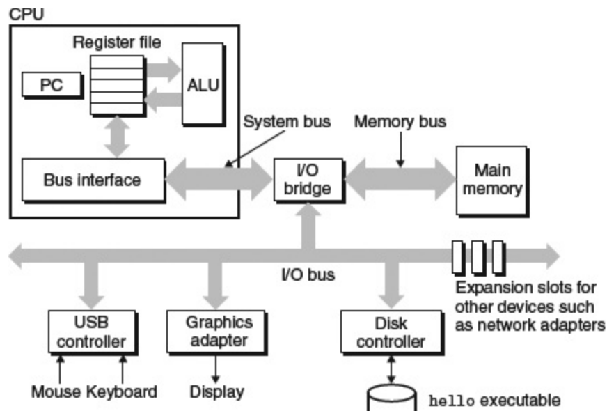
Figure 1.4 Hardware organization of a typical system.
