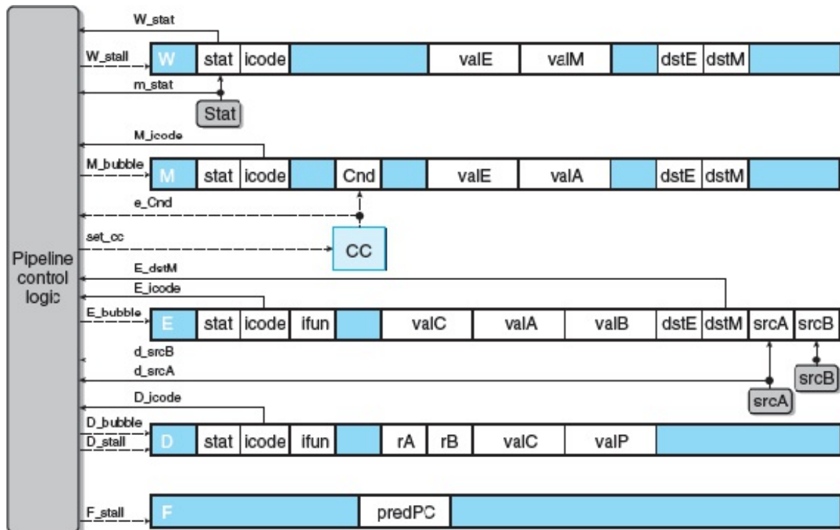
Figure 4.68 PIPE pipeline control logic.
