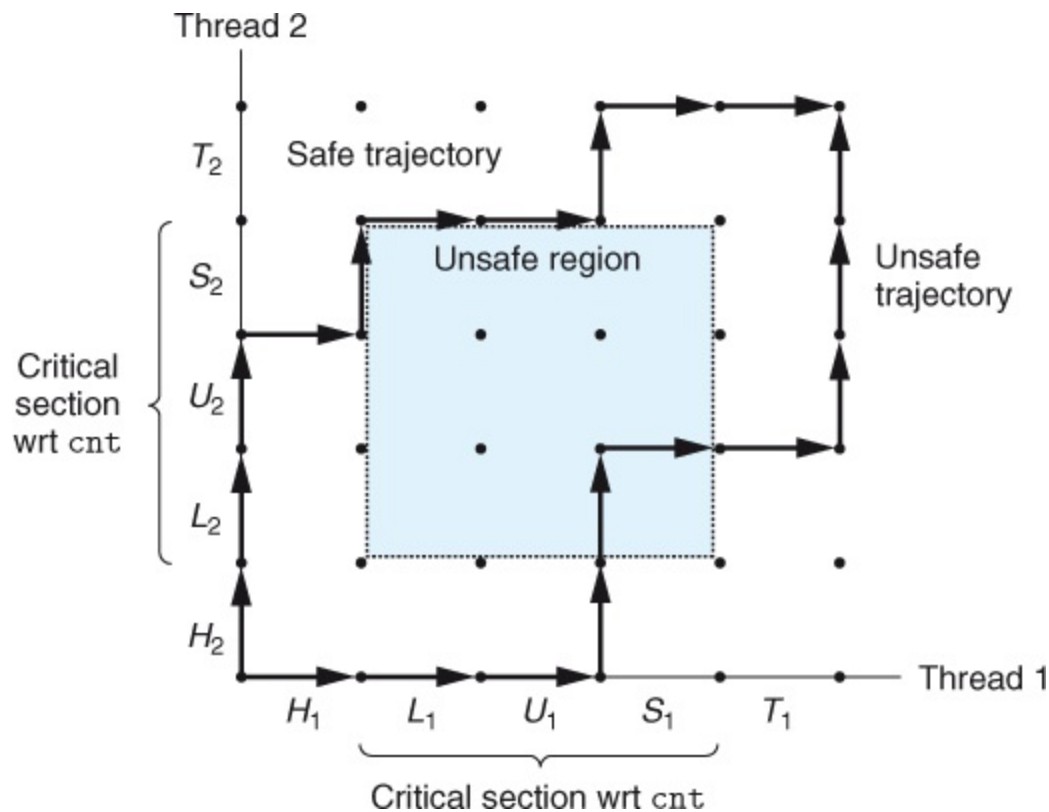
Figure 12.21 Safe and unsafe trajectories.
