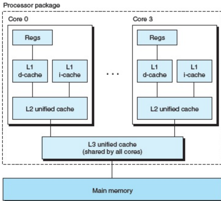
Figure 1.17 Multi-core processor organization.
