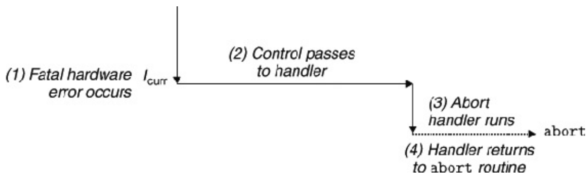
Figure 8.8 Abort handling.
