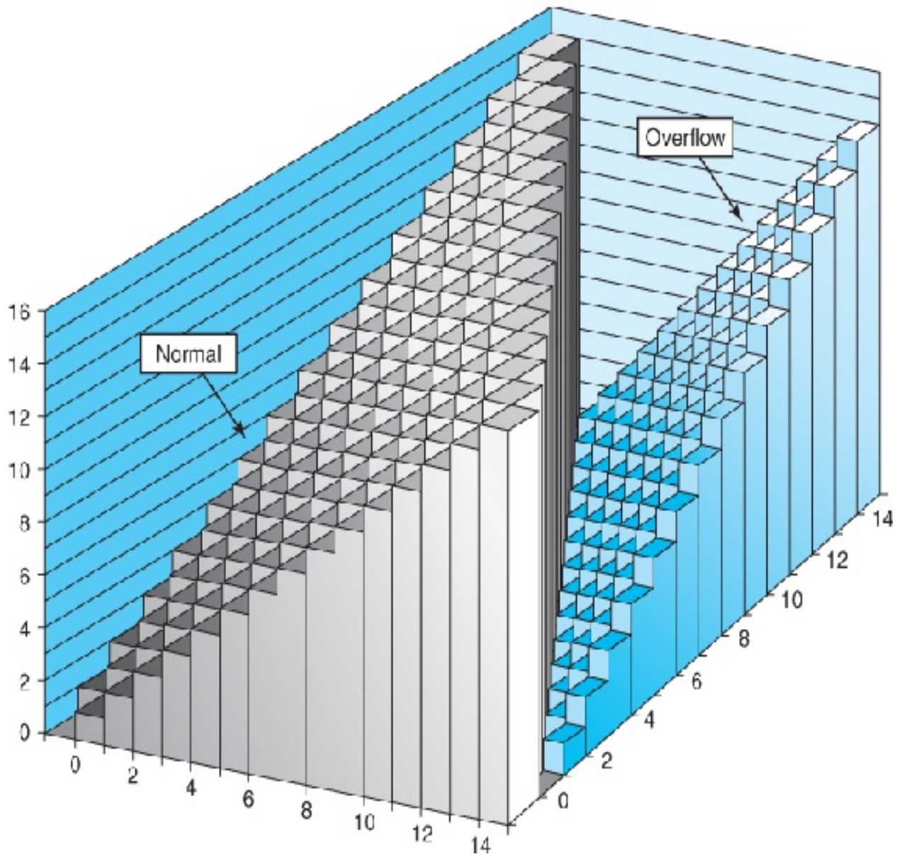
Figure 2.23 Unsigned addition.
