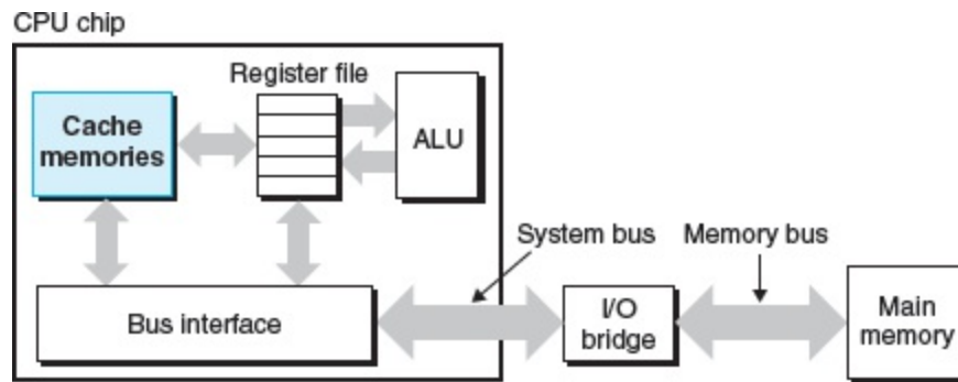
Figure 1.8 Cache memories.
