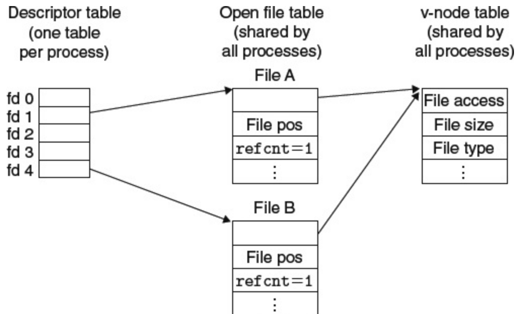
Figure 10.13 File sharing.
