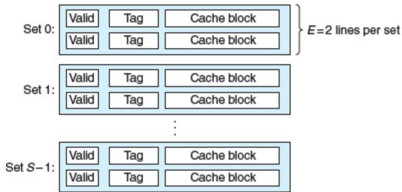
Figure 6.32 Set associative cache ( 1 < E < C/B ).
