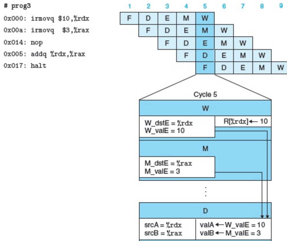
Figure 4.50 Pipelined execution of prog3 using forwarding.
