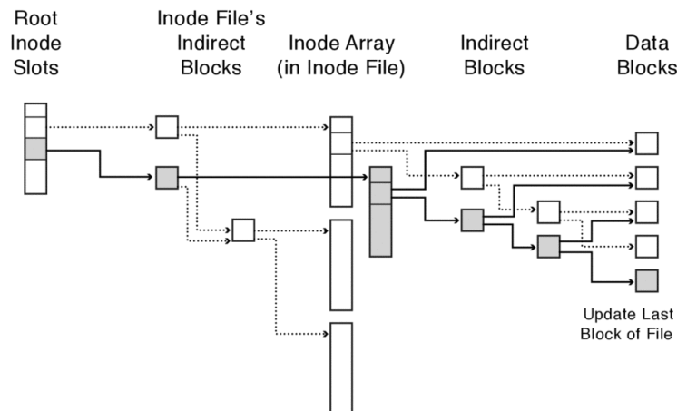
Figure 13.22: In a COW file system, writing a data block causes the system to allocate new blocks for and to write the data block and all nodes on the path from that data block to the root inode.
