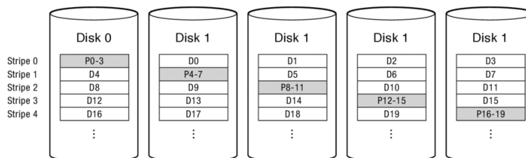
Figure 14.9: RAID 5 with rotating parity.
