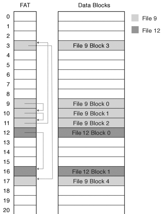
Figure 13.9: A FAT file system with one 5-block file and one 2-block file.
