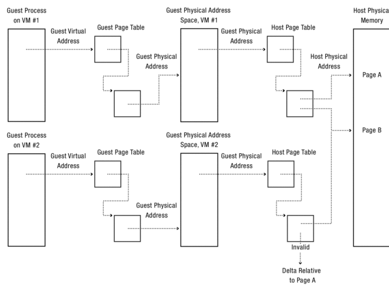
Figure 10.5: When a host kernel runs multiple virtual machines, it can save space by storing a delta to an existing page
