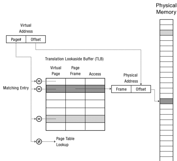
Figure 8.10: Operation of a translation lookaside buffer. In the diagram, each virtual page number is checked against all
