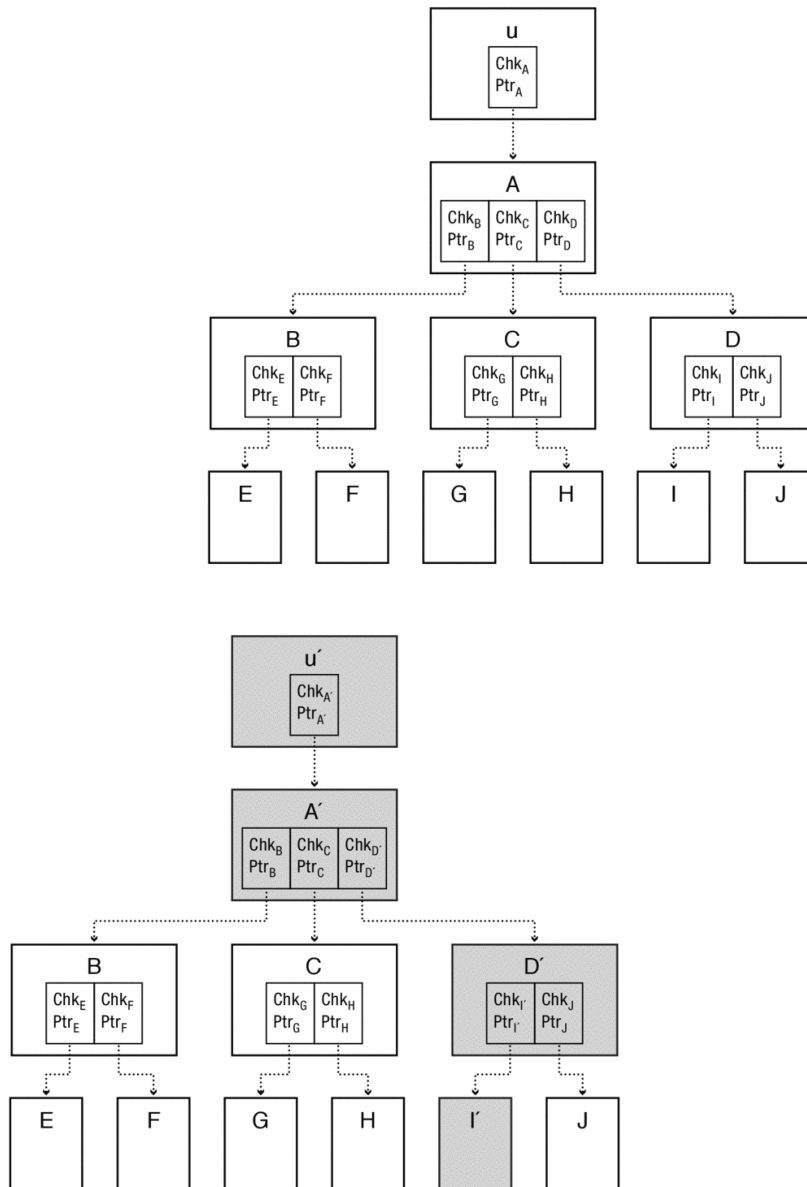
Figure 14.11: ZFS stores all data in a Merkle tree so that each node of the tree includes both a pointer to and a checksum of each of its children (Chk and Ptr in the figure). On an update, all nodes from the updated block (I') to the root (u') are changed to reflect the new pointer and checksum values.
