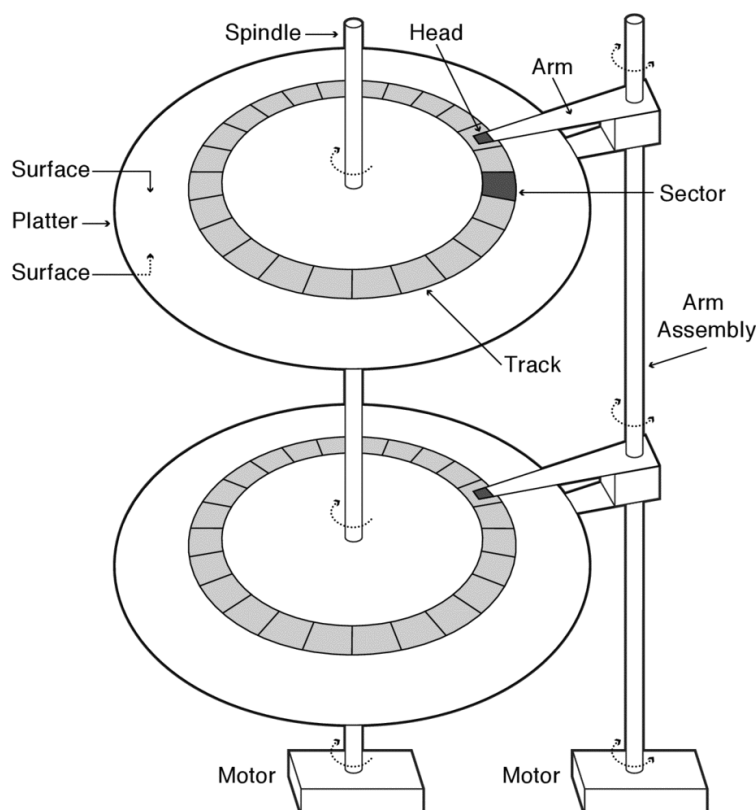
Figure 12.2: Key components of a magnetic disk drive.
