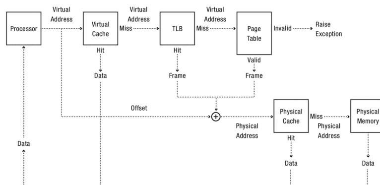
Figure 8.17: Combined operation of a virtually addressed cache, translation lookaside buffer, hardware page table, and physically addressed cache.
