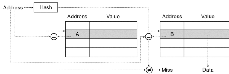
Figure 9.11: Set associative cache lookup. The cache hashes the address to determine which location to check. The cache checks the entry in each table in parallel. It returns the value if any of the entries match the address.
