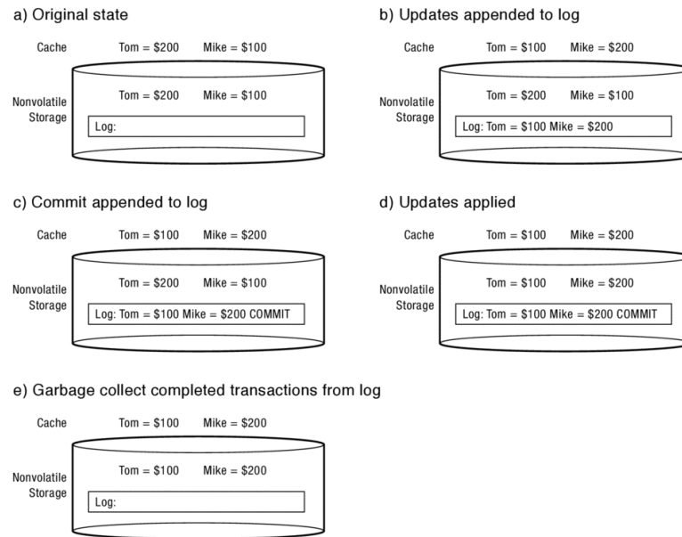
Figure 14.3: Example transaction with redo logging.
