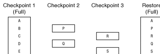
Figure 10.7: The operating system can recover the state of a memory segment after a crash by saving a sequence of incremental checkpoints.
